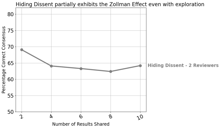
Figure 3. The percentage of runs correct consensus is reached as the amount of evidence considered for publication increases, with exploration. T = 100 , r = 2 , \epsilon = 0.05 .
