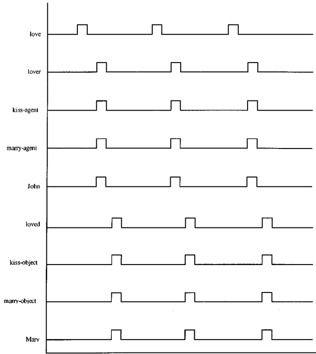
Figure 3. Synchronous oscillation representations of relational instances love(John, Mary), kiss(John, Mary), and marry(John, Mary).
