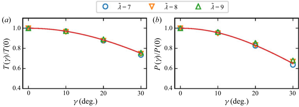
Figure 3. Influence of yaw angle \gamma on the rotor’s thrust and power: (a) the normalized thrust T(\gamma)/T(0) (symbols) compared with \cos^2 \gamma (solid line); and (b) the normalized power P(\gamma)/P(0) (symbols) compared with \cos^3 \gamma (solid line). Here, T(0) and P(0) are the thrust and the power at \gamma = 0 , respectively.
