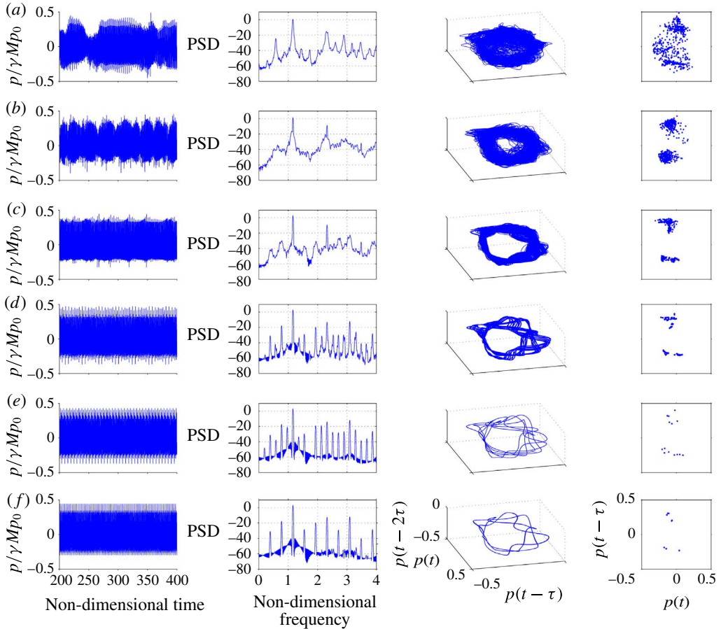
FIGURE 14. (Colour online) Synchronization of a strange attractor: the forced response of the system during chaotic oscillations (state D) when forced at the dominant frequency of its unforced spectrum, f_f/f_n = 1 , where f_n = 1.16 . Time series, power spectra, phase portraits and Poincaré maps are shown for increasing forcing amplitudes: (a) \epsilon \equiv u_f/U_0 = 0.00 or unforced, (b) 0.09, (c) 0.18, (d) 0.27, (e) 0.30 and (f) 0.31.
