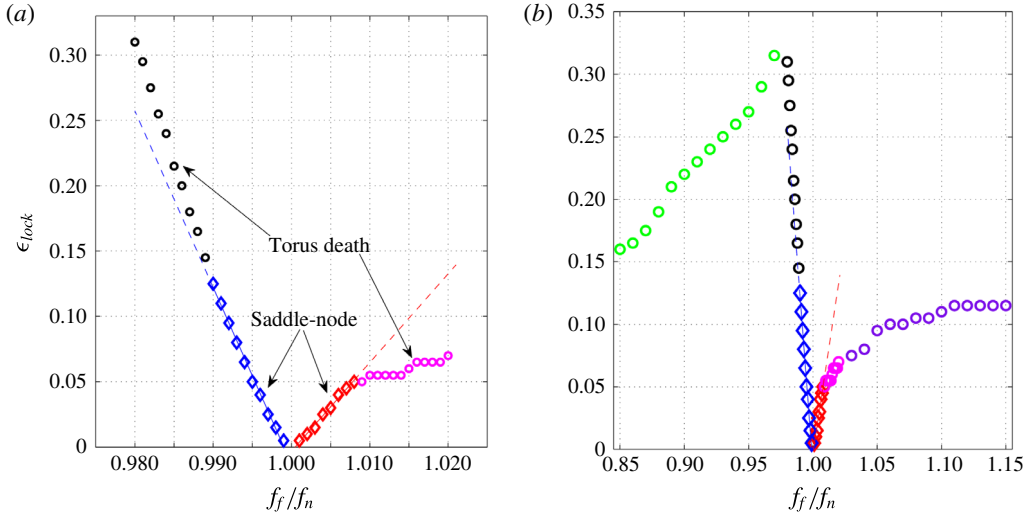
FIGURE 7. (Colour online) The 1 : 1 Arnold tongue for period-1 oscillations (state B) when forced across (a) a small range of frequency detuning ( 0.98 < f_f/f_n < 1.02 ) and (b) a large range of frequency detuning ( 0.85 < f_f/f_n < 1.15 ). The diamond markers denote saddle-node bifurcations, and the circular markers denote torus-death bifurcations. The dashed lines are linear fits to the saddle-node data on either side of f_f/f_n = 1 .
