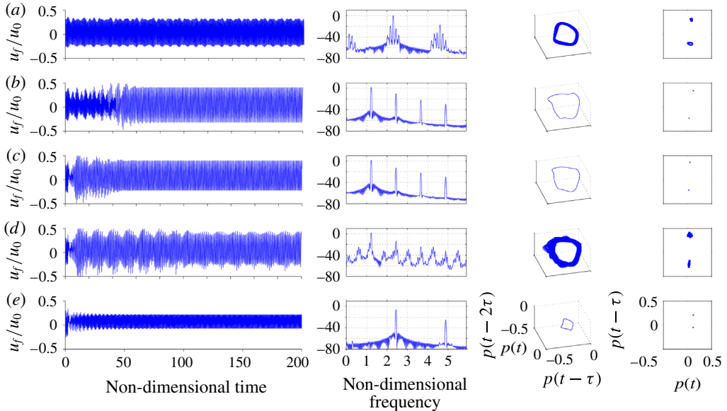
FIGURE 12. (Colour online) Switching between different stable attractors after lock-in: the forced response of the system during period-1 oscillations (state A) when f_f/f_n = 1.06 , where f_n = 2.304 . Time series, power spectra, phase portraits and Poincaré maps are shown for increasing forcing amplitudes: (a) \epsilon \equiv u_f/U_0 = 0.03 , (b) 0.16, (c) 0.18, (d) 0.21 and (e) 0.24.
