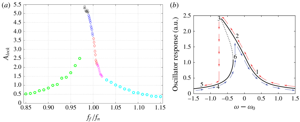
FIGURE 8. (Colour online) (a) The system response at lock-in, i.e. at the critical forcing amplitude, \epsilon_{lock} . The response is defined as the non-dimensional amplitude of the pressure oscillations, A_{lock} = p'/\gamma Mp_0 . As in figure 7(b), the diamond markers denote saddle-node bifurcations, and the circular markers denote torus-death bifurcations, with the different colours indicating different regimes. (b) The frequency-response curve for a forced Duffing oscillator with a soft cubic spring. The dashed branch (between points 3 and 6) is unstable and cannot be reached in experiments or simulations, leaving a discontinuous jump that resembles that seen in panel (a).
