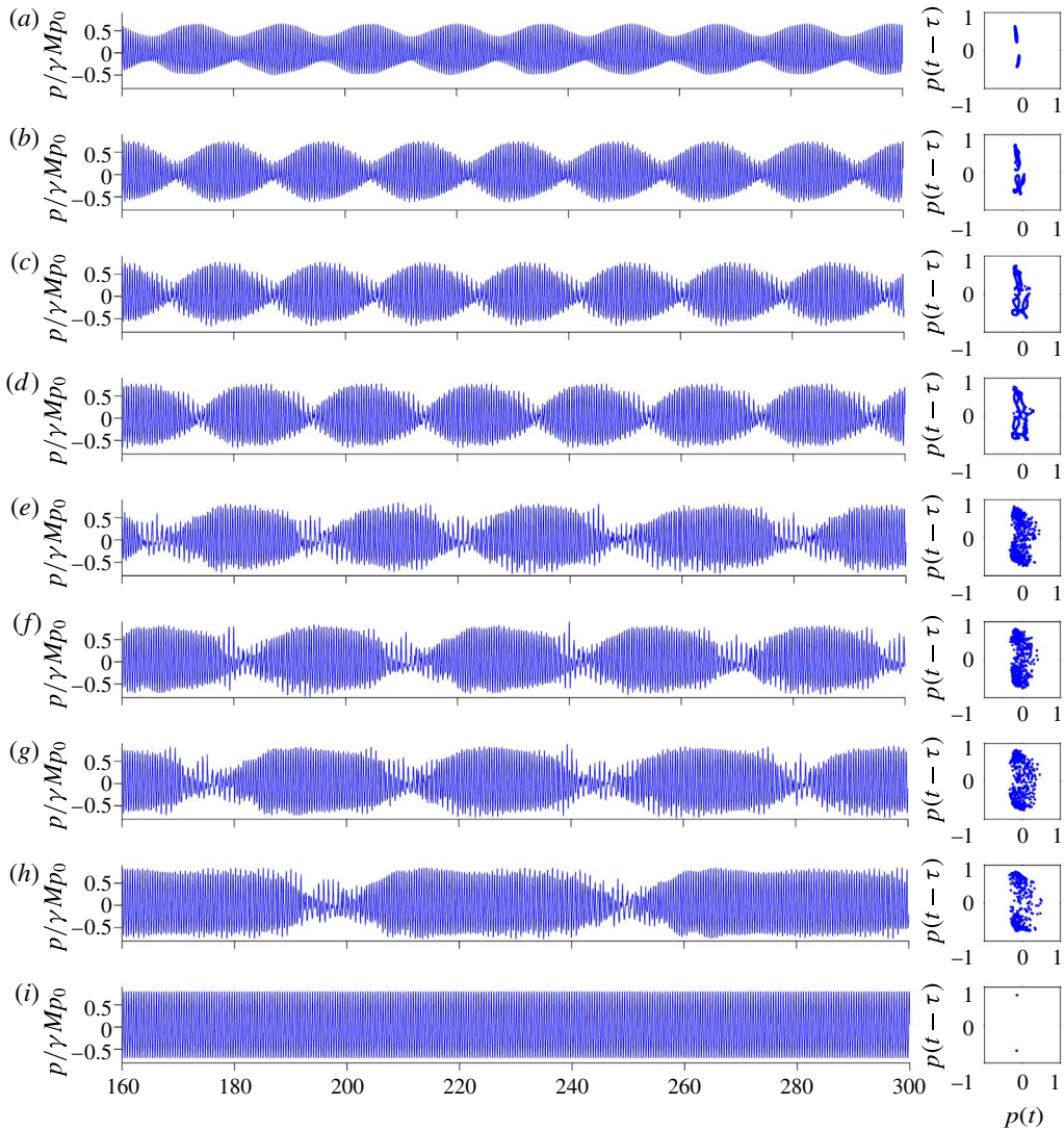
FIGURE 9. (Colour online) Intermittency route to lock-in: the forced response of the system during period-1 oscillations (state A) when f_f/f_n = 0.97 , where f_n = 2.304 . Time series and Poincaré maps are shown for increasing forcing amplitudes: (a) \epsilon \equiv u'_f/U_0 = 0.06 , (b) 0.12, (c) 0.16, (d) 0.18, (e) 0.20, (f) 0.21, (g) 0.22, (h) 0.23 and (i) 0.24.
