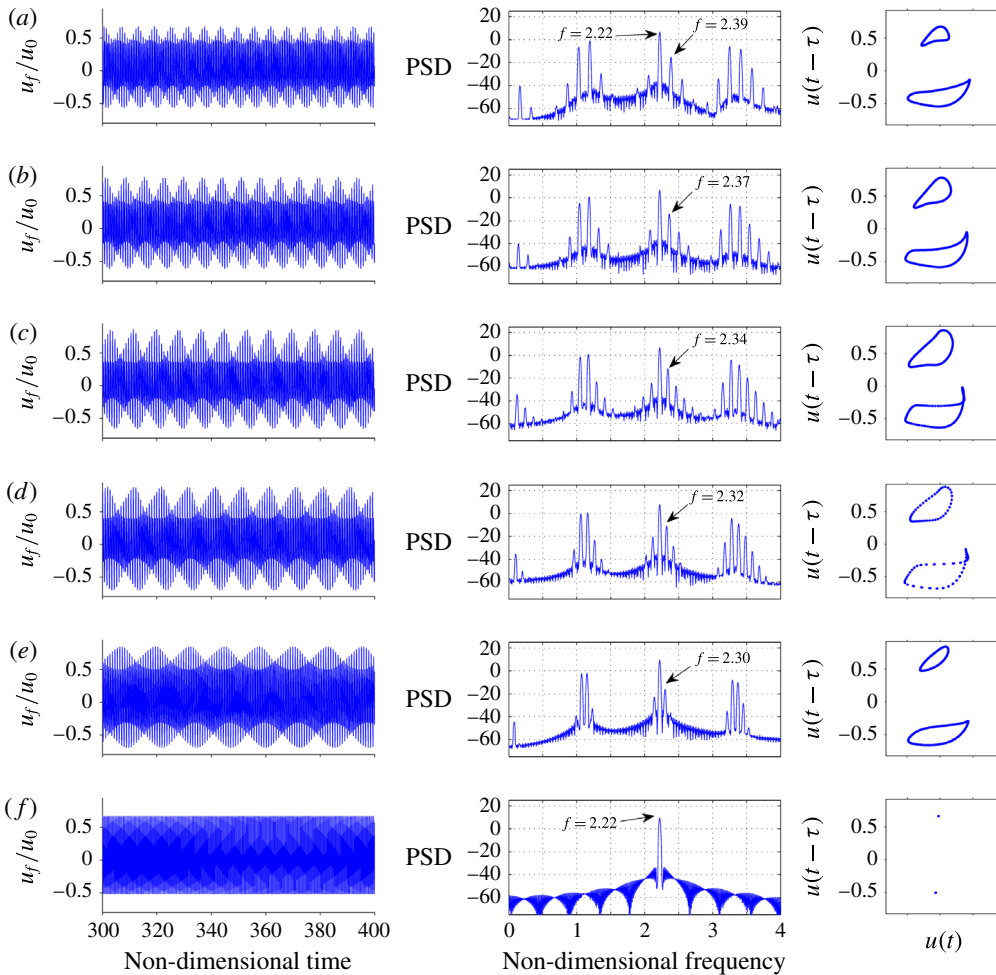
FIGURE 13. (Colour online) Synchronization of a \mathbb{T}^2 attractor: the forced response of the system during quasi-periodic oscillations (state C) when forced at the dominant characteristic frequency of its 2-torus, f_f/f_1 = 1 , where f_1 = 2.22 . Time series, power spectra and Poincaré maps are shown for increasing forcing amplitudes: (a) \epsilon \equiv u_f/U_0 = 0.00 or unforced, (b) 0.09, (c) 0.18, (d) 0.24, (e) 0.30 and (f) 0.31.
