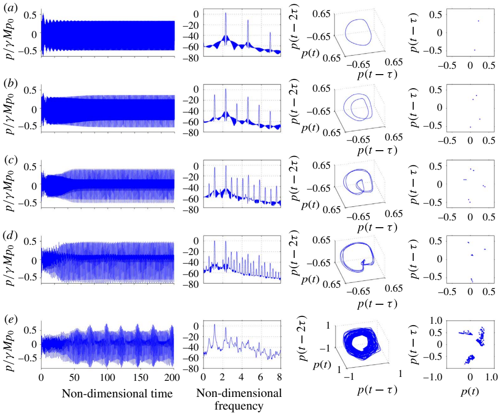
FIGURE 11. (Colour online) Transition to chaos from lock-in via period-doubling bifurcations (route I): the forced response of the system during period-1 oscillations (state B) when f_f/f_n = 1 , where f_n = 1.125 . Time series, power spectra, phase portraits and Poincaré maps are shown for increasing forcing amplitudes: (a) \epsilon \equiv u'_f/U_0 = 0.16 , (b) 0.24, (c) 0.30, (d) 0.34 and (e) 0.36.
