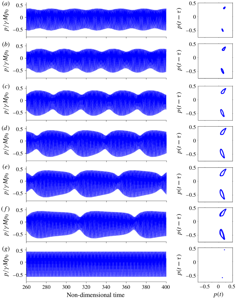
FIGURE 2. (Colour online) Saddle-node bifurcation to lock-in: the forced response of the system during period-1 oscillations (state A) when the forcing frequency is close to the natural frequency, f_f/f_n = 0.98 , where f_n = 2.304 . Time series and Poincaré maps are shown for increasing forcing amplitudes: (a) \epsilon \equiv u_f'/U_0 = 0.03 , (b) 0.06, (c) 0.09, (d) 0.11, (e) 0.12, (f) 0.125 and (g) 0.13.
