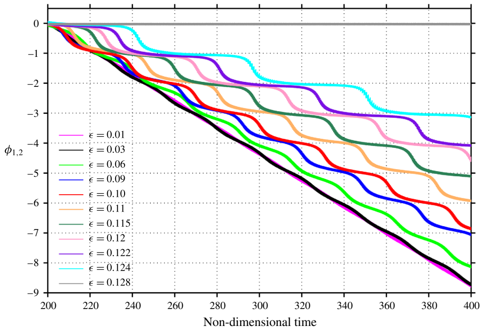
FIGURE 3. (Colour online) Saddle-node bifurcation to lock-in: the phase difference (normalized by 2\pi ) between the system and the forcing at the conditions of figure 2.
