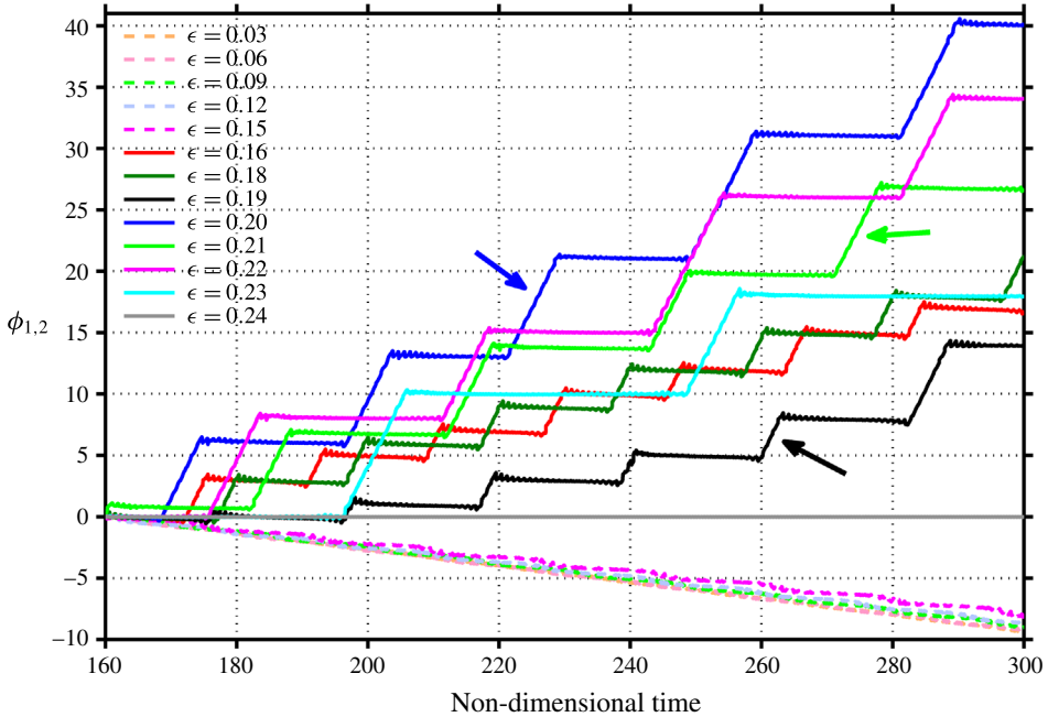
FIGURE 10. (Colour online) Intermittency route to lock-in: the phase difference (normalized by 2\pi ) between the system and the forcing at the conditions of figure 9. The arrows show that phase slips can be greater than 2\pi .
