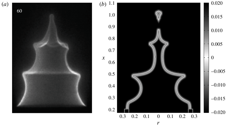
FIGURE 1. Flame wrinkling due to vortex formation and roll-up. (a) Experimental image of a forced conical flame. (Reprinted from Karimi et al. (2009) with permission from Elsevier.) (b) The G -field obtained from numerical simulations of a forced conical flame. (Reprinted from Orchini et al. (2015) with permission from Cambridge University Press.) In both cases, the forcing is harmonic, with the same frequency and amplitude. The flame contour G=0 is highlighted to show that it can qualitatively reproduce the experimental results.
