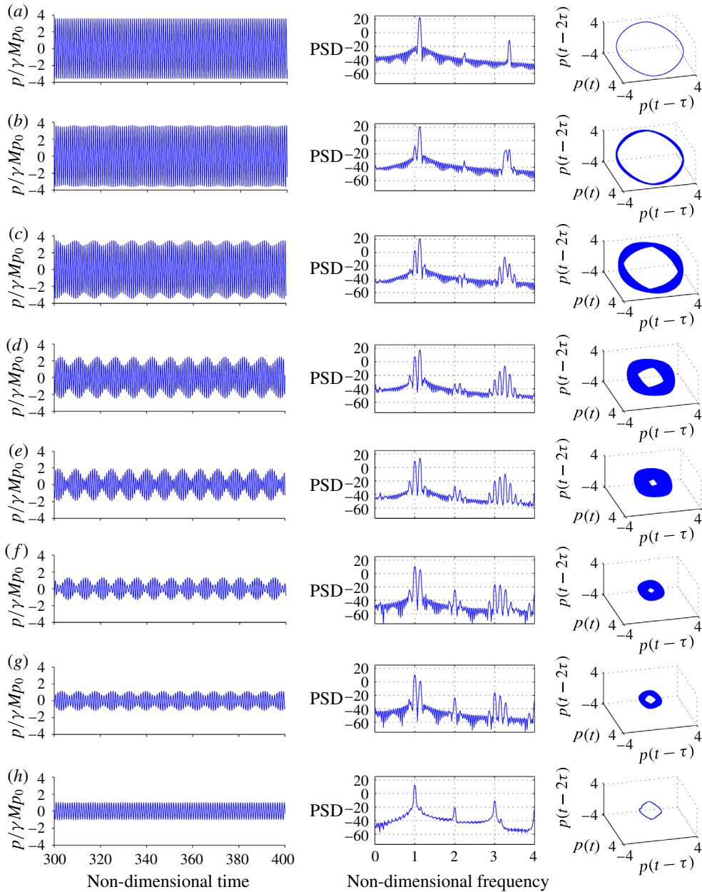
FIGURE 4. (Colour online) Torus-death bifurcation to lock-in: the forced response of the system during period-1 oscillations (state B) when the forcing frequency is far from the natural frequency, f_f/f_n = 0.89 , where f_n = 1.125 . Time series, power spectra and phase portraits are shown for increasing forcing amplitudes: (a) \epsilon \equiv u_f/U_0 = 0.00 or unforced, (b) 0.02, (c) 0.08, (d) 0.14, (e) 0.16, (f) 0.18, (g) 0.20 and (h) 0.23.
