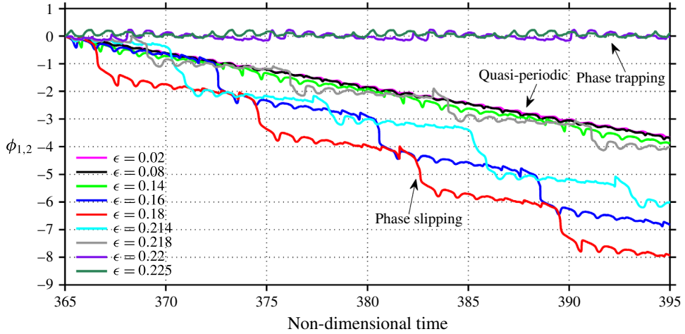
FIGURE 5. (Colour online) Torus-death bifurcation to lock-in: the phase difference (normalized by 2\pi ) between the system and the forcing at the conditions of figure 4.
