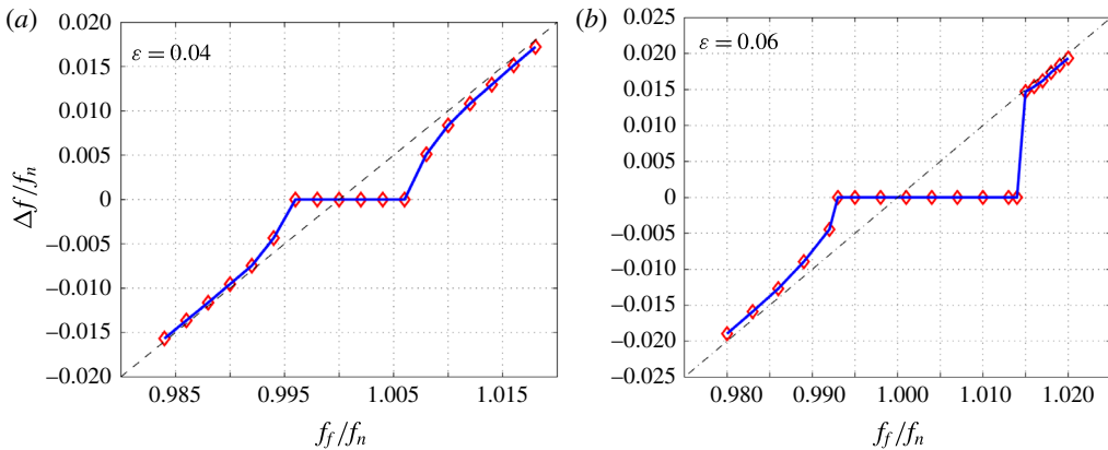
FIGURE 6. (Colour online) Dependence of the beating frequency, \Delta f = f_f - f'_n , on the forcing frequency, f_f , both normalized by the unforced natural frequency, f_n , at two forcing amplitudes: (a) \epsilon = 0.04 , where lock-in occurs via a saddle-node bifurcation for both f_f < f_n and f_f > f_n , and (b) \epsilon = 0.06 , where lock-in occurs via a saddle-node bifurcation for f_f < f_n but via a torus-death bifurcation for f_f > f_n .
