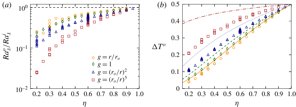
FIGURE 4. (Colour online) (a) Ratio of boundary layer Rayleigh numbers (3.4) for various radius ratios and gravity profiles. The horizontal dashed line corresponds to the hypothetical identity Ra_{\lambda}^i = Ra_{\lambda}^o . (b) Temperature drop at the outer boundary layer. The lines correspond to the theoretical prediction given in (3.5).
