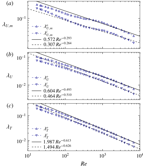
FIGURE 15. (Colour online) (a) Viscous boundary layer thicknesses at the outer boundary ( \lambda_{U,m}^i ) and at the inner boundary ( \lambda_{U,m}^o ) as a function of the Reynolds number for the cases of table 1 ( \eta = 0.6 , g = (r_o/r)^2 ). (b) Same for the alternative definition of the viscous boundary layer, i.e. \lambda_U^i and \lambda_U^o . (c) Thermal boundary layer thicknesses at the outer boundary ( \lambda_T^i ) and at the inner boundary ( \lambda_T^o ) as a function of Re . The black lines in (a–c) correspond to the least-squares fit to the data for the numerical models with Ra \geq 10^6 (i.e. Re > 250 ).
