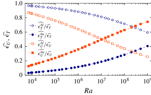
FIGURE 23. (Colour online) Estimated relative contributions of the boundary layer (open symbols) and the fluid bulk (filled symbols) to \hat{\epsilon}_U (orange squares) and \hat{\epsilon}_T (blue circles) using (5.13).
