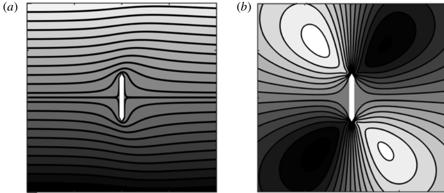
FIGURE 6. The basic symmetric flow regime at \beta = 300 , KC = 0.2 . (a) Instantaneous streamlines at t/T - T_0 = 0 ( T_0 = 30 ), (b) streamlines of the secondary flow.
