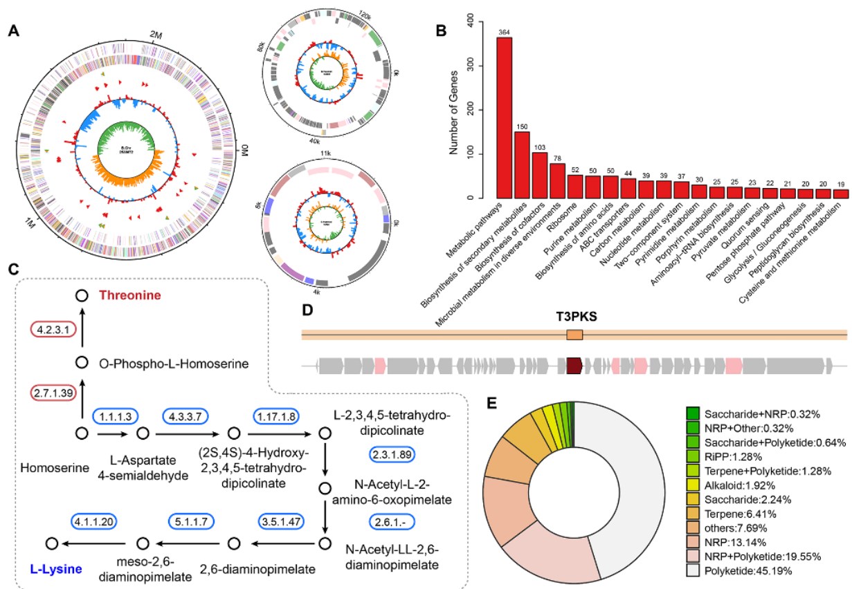
Figure 2. Genome information of L. reuteri ZJ617. (A) Circular genomic map of L. reuteri ZJ617 chromosome and two plasmids. from the outermost to innermost circle, circle 1 represents genome size; circles 2 and 3 are forwards CDSS and reverse CDSS, respectively, color-coded according to the COG classification; circles 4 is rRNA genes and tRNA genes; circles 5 represents GC content; circles 6 is GC skew. (B) The bar of KEGG pathway. (C) threonine and l-lysine biosynthesis pathway. (D) the secondary metabolite BGCs. (E) the classification of GCFs.
