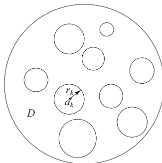
FIGURE 1. Multiply connected domain D with circular boundaries.
