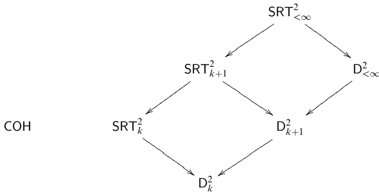
FIGURE 2. Relationships between \text{SRT}_k^2 , D_k^2 , and \text{COH} , with k \geq 2 arbitrary. All arrows represent reductions under \leq_{\text{sw}} . No additional arrows hold under either \leq_{\text{w}} or \leq_{\text{sc}} .
