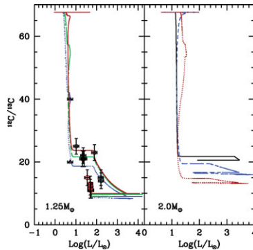
Figure 3. Evolution of the surface ^{12}\text{C}/^{13}\text{C} value as a function of stellar luminosity for models of 1.25 and 2 M_{\odot} stars (left and right respectively). Different tracks are for different initial rotation velocities ( 50 , 80 , and 110 \text{ km.s}^{-1} for the 1.25 M_{\odot} star, and 0 , 110 , and 250 \text{ km.s}^{-1} for the 2 M_{\odot} star). Observations by Gilroy & Brown (1991) in evolved stars of the open cluster M67 (turnoff mass \sim 1.2 M_{\odot} ) are also shown (triangle, squares, and circles for subgiant, RGB, and clump stars respectively). Adapted from Lagarde & Charbonnel (in preparation)
