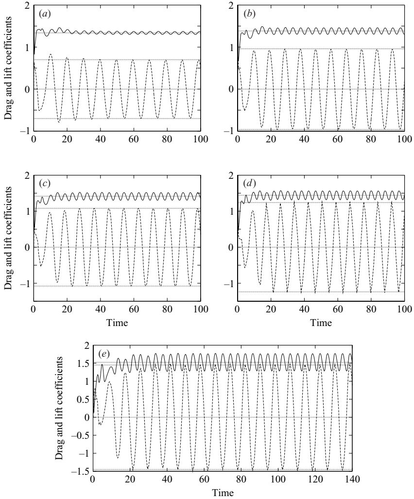
FIGURE 2. Drag and lift coefficients at Re = (a) 200, (b) 300, (c) 400, (d) 500 and (e) 1000 . —, C_D ; - -, C_L ; ···, values from table 1.
