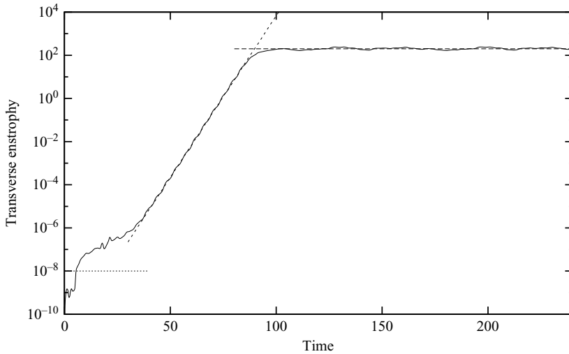
FIGURE 7. Development of transverse enstrophy Z^\perp = (\|\omega_x\|_2^2 + \|\omega_y\|_2^2)/2 at Re = 400 . Dashed lines show the constant value 200 and the exponential a e^{t/2.9} with a = 7.41 \times 10^{-12} .
