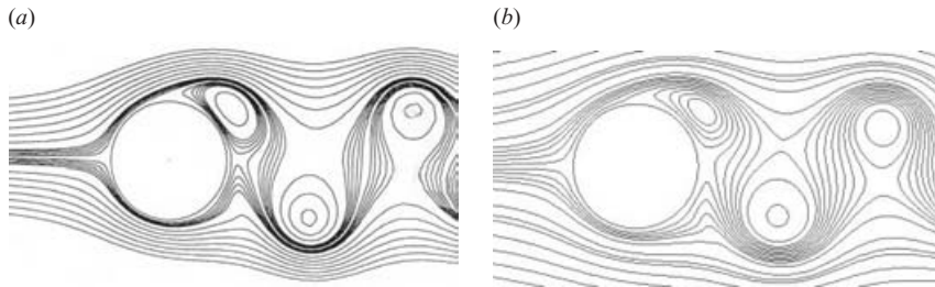
FIGURE 4. Streamlines at Re = 500 for A = 3/\pi and S_F = 1/3 \simeq 1.45S_t , obtained by (a) Dennis et al. (2000), and (b) the present work. Part (a) was kindly provided by S.C.R. Dennis.
