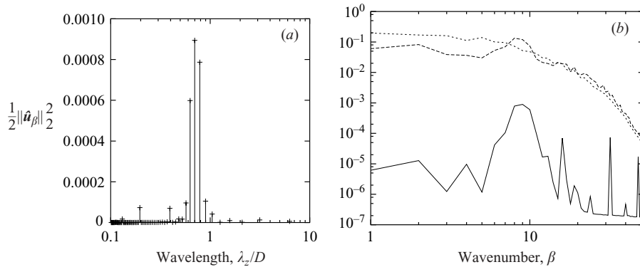
FIGURE 6. Axial energy spectrum at Re = 400 . (a) Energy spectrum with respect to \lambda_z/D and its resonance at \lambda_z/D \simeq 0.73 , at t = 60 during the transient from two and to three-dimensions. (b) Energy spectra with respect to the modes \beta at t = 60 (—), t = 100 (---) and t = 150 (- - -).
