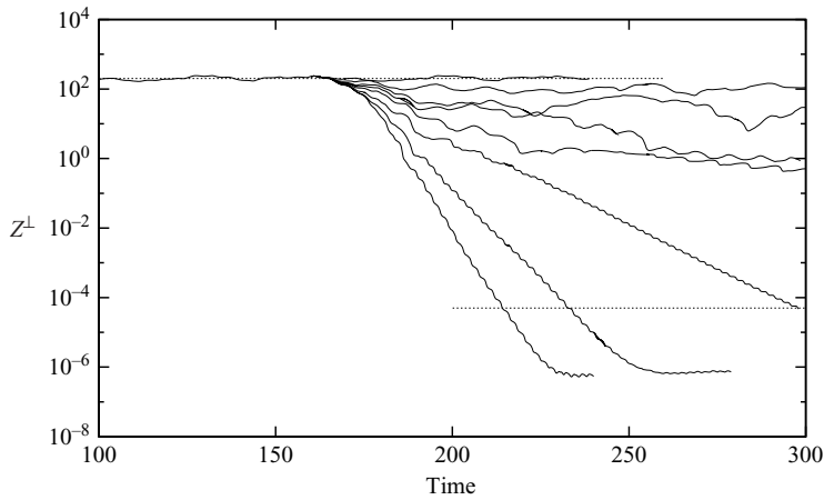
FIGURE 15. Transverse enstrophy Z^\perp at Re = 400 with respect to time, for several rotation amplitudes, in a logarithmic scale. From bottom to top: A = \pi/2 , A = 2\pi/5 , A = \pi/3 , A = 2\pi/7 , A = \pi/3.75 , A = \pi/4 , A = \pi/5 and A = 0 (steady).
