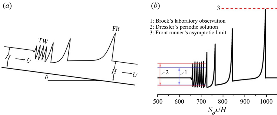
Figure 2. (a) A roll-wave group characterized by a FR and a pack of TWs. (b) The roll-wave group produced by a local disturbance in one simulation.
