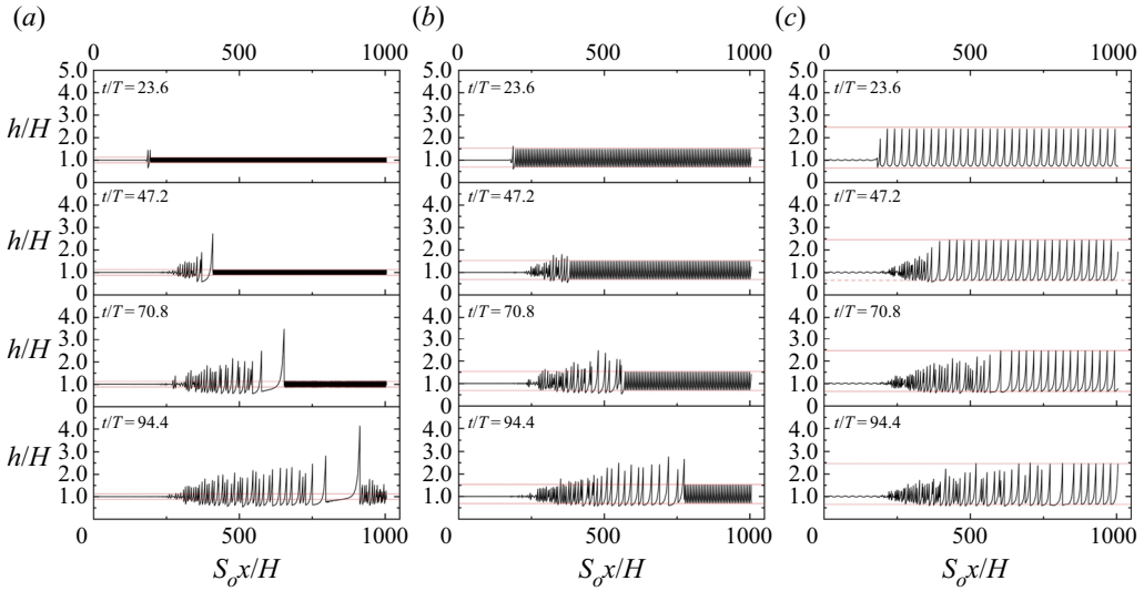
Figure 13. Roll waves due to uniform flow at the inlet on a periodic channel bed. The channel slope is perturbed with an amplitude \epsilon_B = 0.10 and wavelength S_0 \lambda_B/H = (a) 1.57, (b) 6.28 and (c) 25.12. The normal-flow Froude number in this series of simulations was Fr = 3.71 .
