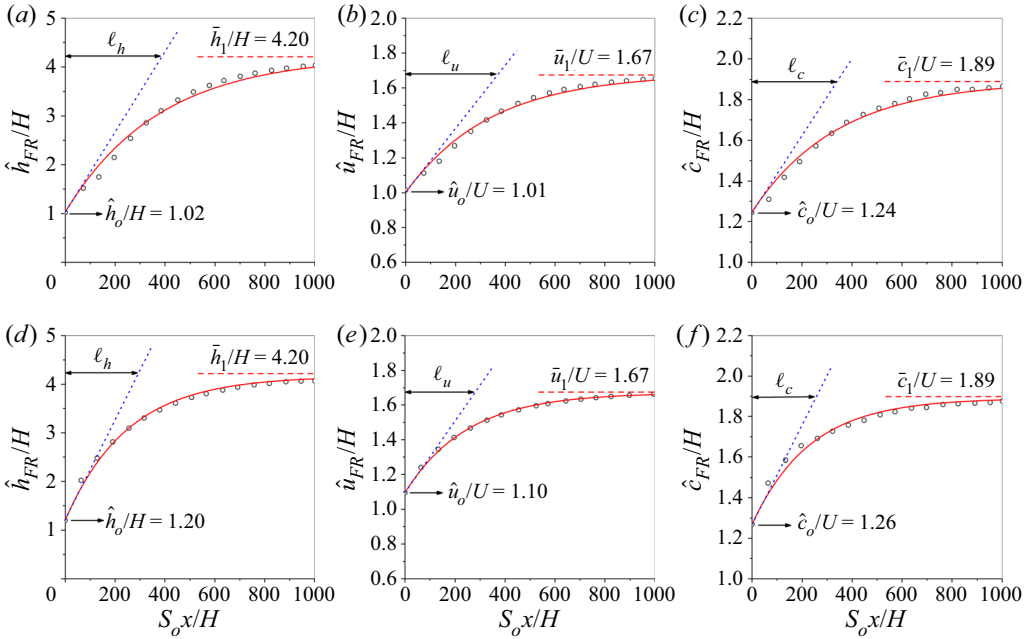
Figure 8. The approach of the FR towards its asymptotic state for Fr = 3.71 . The dotted line delineates the initial growth rate. The dashed line defines the asymptotic state. For \epsilon = 0.02 , the best fit to the simulation data gives (a) \ell_h = 377 , (b) \ell_u = 348 and (c) \ell_c = 356 . For \epsilon = 0.2 , the best fit to the simulation data gives (d) \ell_h = 241 , (e) \ell_u = 248 and (f) \ell_c = 223 .
