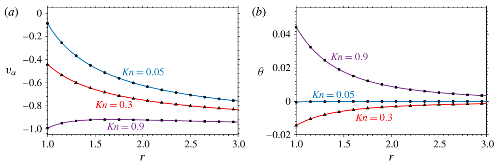
FIGURE 3. The polar velocity v_\alpha at \alpha = \pi/2 and temperature \theta at \alpha = 0 for flow around a sphere. The R13-MFS predictions ( \bullet , \blacktriangle , \blacksquare ) for Kn = 0.05, 0.3, 0.9 respectively compared with the analytic result from Torrilhon (2010) (solid lines).
