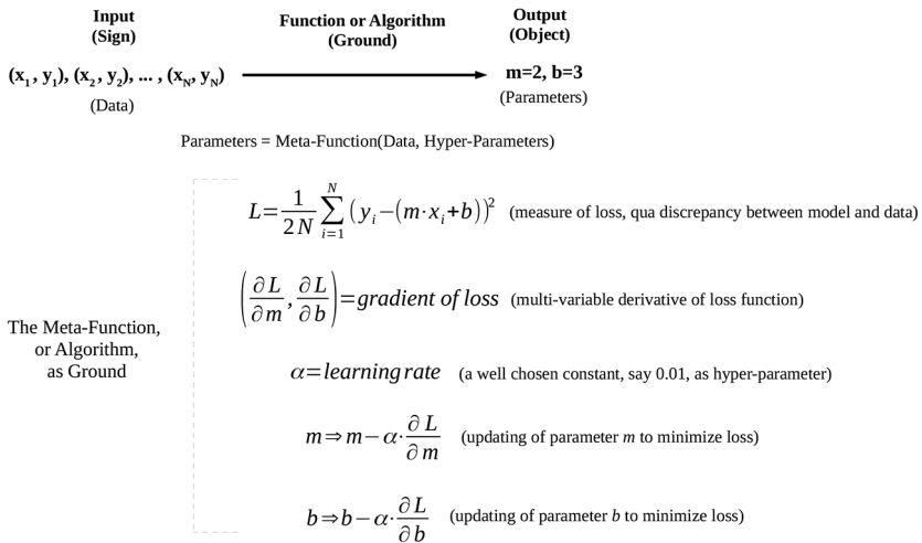
Figure 4. Gradient descent
