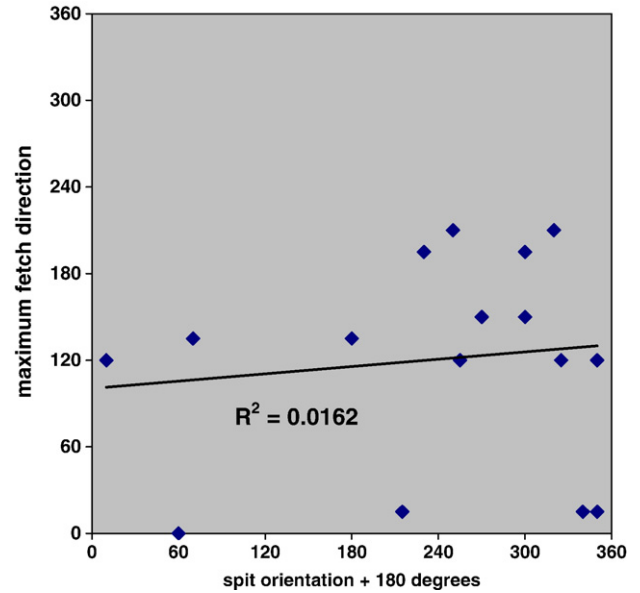
Figure 6. Spit orientation + 180° plotted against direction of maximum fetch for all 17 spits in the central portion of Bonneville basin. The poor correlation between the two indicates that fetch is not an important factor in determining spit orientation.
