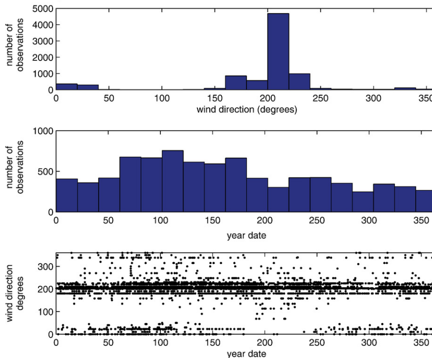
Figure 7. Summary of strong modern winds at Salt Lake International Airport and Milford, Utah. Data are winds > 10 m/s for a period in which the 12-h average wind was > 5 m/s. The period analyzed was 1946–1993.
