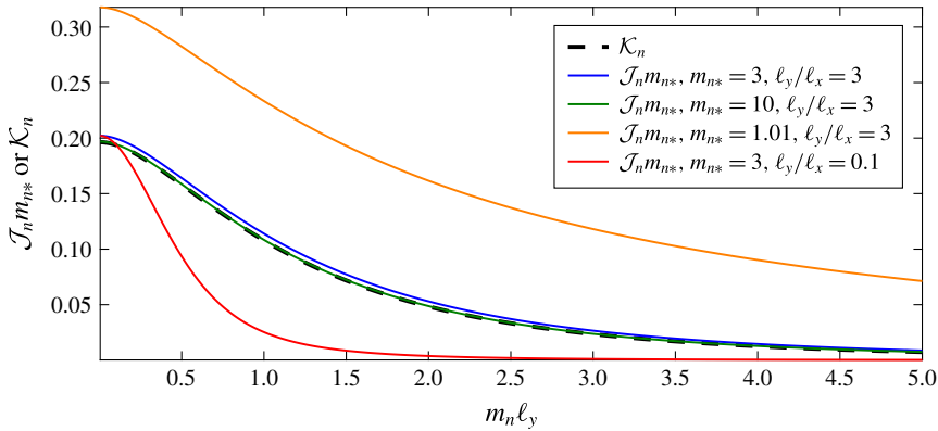
FIGURE 7. (Colour online) The approximate dimensionless integral \mathcal{K}_n (dashed) compared with exact solutions \mathcal{J}_n m_{n*} (solid) over a range of the control parameters m_n \ell_y . The approximation agrees well in two cases where the assumptions ( m_{n*}^2 \gg 1 and \ell_y > \ell_x ) are met (blue and green). The approximation is very poor when the assumptions are not met (orange and red).
