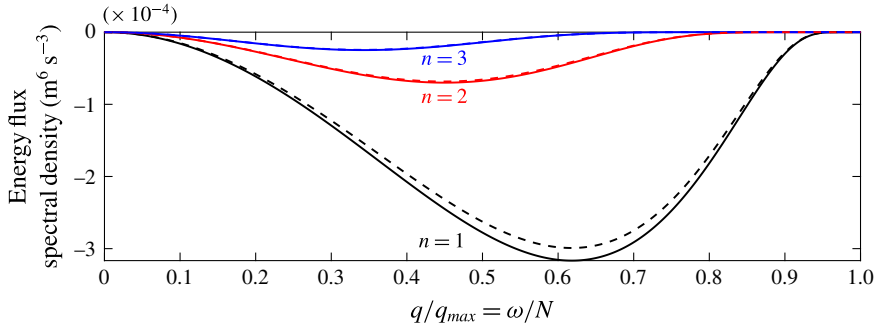
FIGURE 6. (Colour online) The energy flux spectral density for the typical SW and stratification parameters in table 1. The solid lines show the exact integrand in (4.13), and the dashed lines show the approximation in (4.20) for the first three vertical modes as a function of normalized horizontal wavenumber, q/q_{max} , which is equivalent to the IW frequency, \omega , normalized by the buoyancy frequency N .
