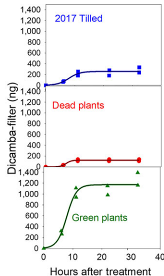
Figure 1. Dicamba emissions in 2017 as affected by surface condition and hours after treatment presented as cumulative nanograms. Regression equation set to y = a/(1 + \exp(-(\text{hours} - c)/b)) . Parameter a = maximum dicamba at asymptote, parameter c = time in hours to reach inflection point of curve where dicamba concentration is increasing at a slower rate. Regression parameters are given in Table 3.
