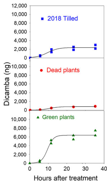
Figure 2. Dicamba emissions in 2018 as affected by surface condition and hours after treatment presented as cumulative nanograms. Regression equation set to y = a/(1 + \exp(-(\text{hours} - c)/b)) . Parameter a = maximum dicamba at asymptote, parameter c = time in hours to reach inflection point of curve where dicamba concentration is increasing at a slower rate. Regression parameters are given in Table 3.
