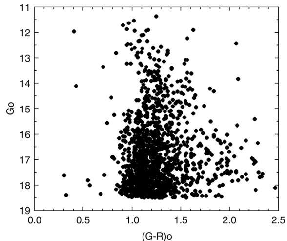
Figure 3 Colour-magnitude diagram for the field down to the limiting magnitude, G = 18.5 .
