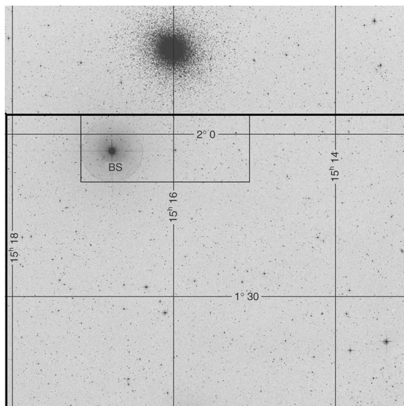
Figure 2 The field chart showing the position of the cluster M5, the bright star HD 136202 ( \alpha = 15^{\text{h}} 19^{\text{m}} 18^{\text{s}}.80 , \delta = +01^{\circ} 45' 55''.5 ), labelled with BS, and the surrounding excluded area of 0.104 \text{ deg}^2 . The horizontal and vertical axes give the right ascension \alpha and declination \delta , respectively.
