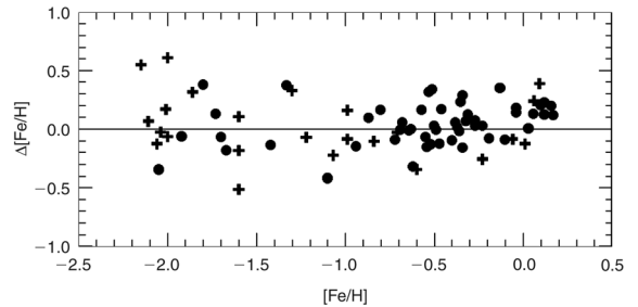
Figure 13 \Delta[\text{Fe}/\text{H}] versus metallicity, where \Delta[\text{Fe}/\text{H}] is the difference between the original metallicities and the evaluated ones, utilising the new calibration, [\text{Fe}/\text{H}] = 0.11 - 2.22\delta_{1.08} - 7.95\delta_{1.08}^2 . Symbols: (●) stars from Carney (1979), and (+) stars from Cayrel de Strobel et al. (1997).
