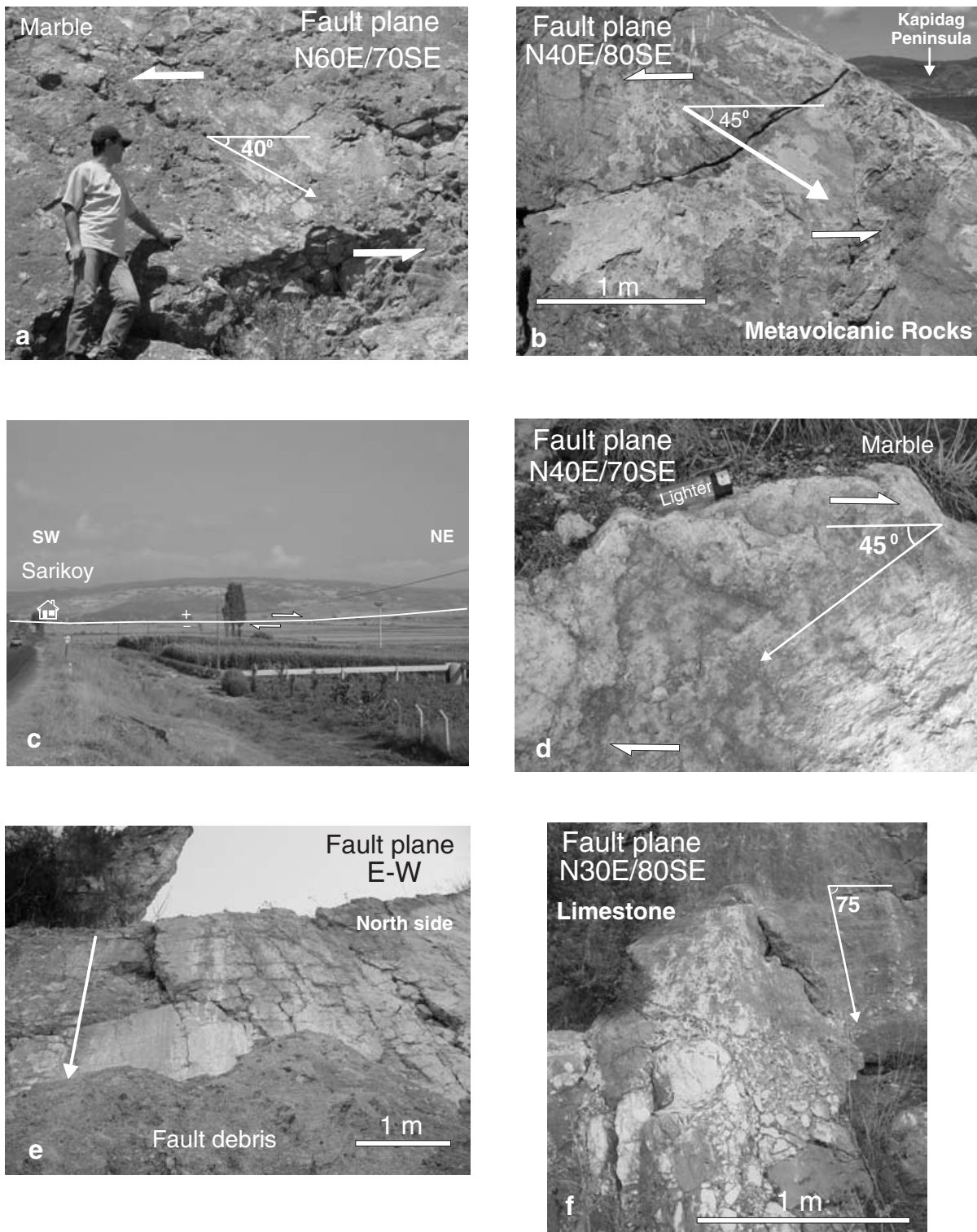
Figure 6. Field photographs of (a) Örtülüce Fault, (b) Dostel Fault, (c) Sarıköy Fault, (d) Gönen Fault, (e) Üçpınar Fault, (f) Biga Fault. Arrows indicate direction of movement.
