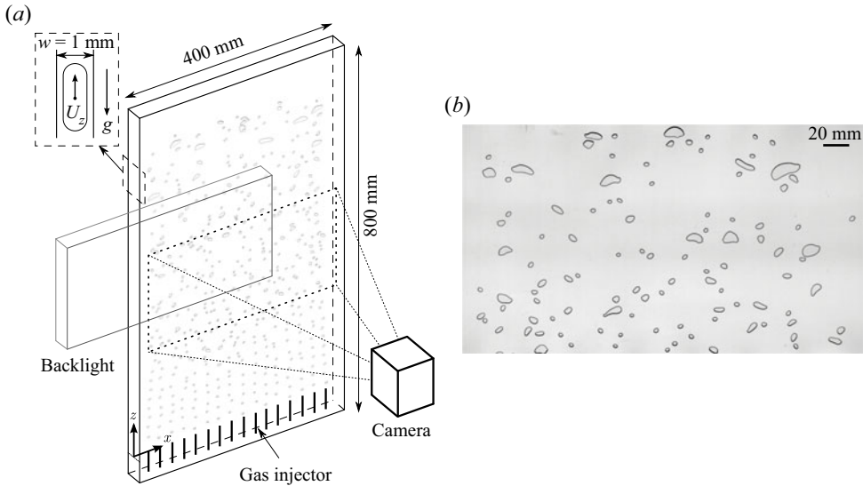
Figure 1. (a) Sketch of the experimental facility, showing the field of view of size 358.40 mm × 179.20 mm for one of the camera recording positions. The zoomed area schematizes the lateral view of the cell with a bubble flattened between the side walls. (b) Example of image taken in one of the three different vertical positions of the camera.
