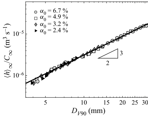
Figure 18. Mean collision frequency \langle h \rangle_{\infty} , averaged over all the bubble sizes present in the swarm at each stage of its evolution, as a function of the corresponding D_{V90} . The values of \langle h \rangle_{\infty} are divided by a constant C_{\infty}(\alpha_0) , where C_{\infty} = 0.163; 0.225; 0.362 and 0.381 for \alpha_0 = 2.4\%; 3.2\%; 4.9\% and 6.7\% , respectively. The thick solid line represents the expression \sqrt{gD_{V90}D_{V90}w} , showing the slope 3/2 as a function of D_{V90} , characteristic of the collisions taking place in the first regime.
