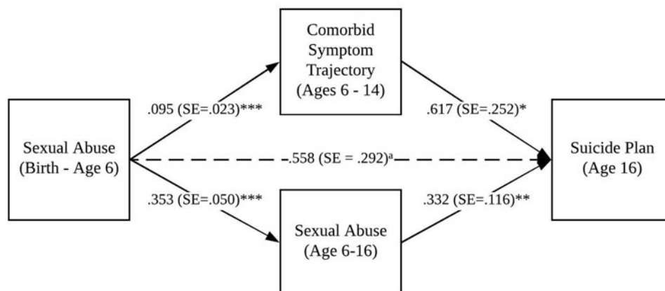
Figure 3. Tests of mediation. Unstandardized parameter estimates are shown in figure. a p < .10 , * p < .05 , ** p < .01 , *** p < .001 .
