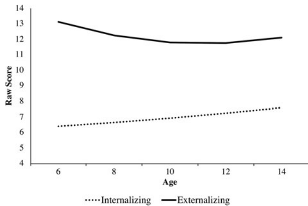
Figure 1. Bivariate growth curve with quadratic terms.
