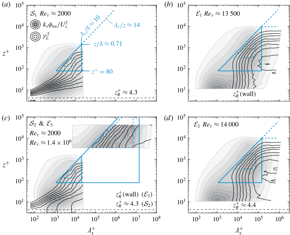
FIGURE 4. Coherence and energy spectrograms, following \gamma_L^2(z, z_R; \lambda_x) (levels: 0.1:0.1:0.9) and k_x \phi_{uu}(z; \lambda_x)/U_\tau^2 (levels: 0.2:0.2:1.8) for all datasets listed in table 1. The triangles (and the regions identified with the dashed lines) are described in § 3.4 (it should be noted that the inner and outer limits of the triangle are listed in panel a).
