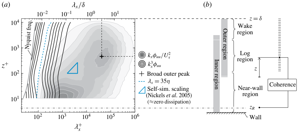
FIGURE 1. (a) Premultiplied energy spectrogram k_x \phi_{uu} / U_\tau^2 (levels: 0.2:0.2:1.8) at Re_\tau \approx 14000 (Baars, Hutchins & Marusic 2017), alongside a spectrogram of the surrogate dissipation k_x^3 \phi_{uu} (at each z , the dissipative spectrum is normalized by its maximum value; levels: 0.15:0.15:0.9). The dashed line closely resembling the ridge in the dissipation spectrogram is \lambda_x = 35\eta , where \eta \equiv (\nu^3/\epsilon)^{1/4} , with \epsilon \equiv 15\nu \int k_x^3 \phi_{uu} d \log(k_x) . (b) Regions in a TBL with a systems diagram depicting the coherence between a reference position, z_R , and a range of z positions.
