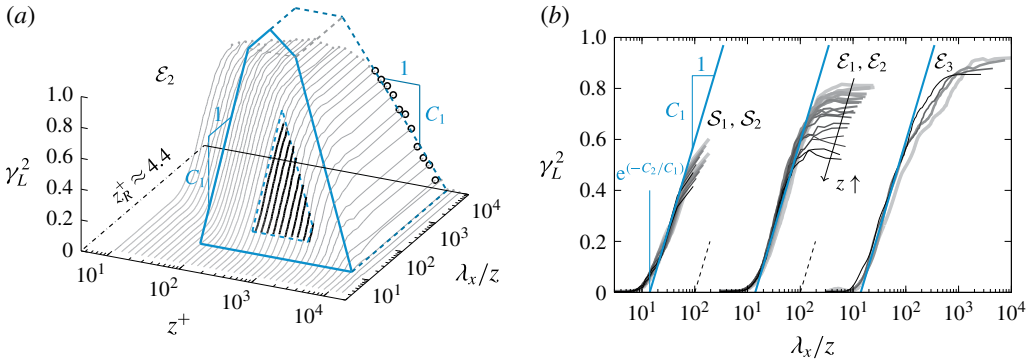
FIGURE 5. (a) Coherence spectrogram of dataset \mathcal{E}_2 (with the wavelength axis predivided by z ). The thicker portions of the curves correspond to 3Re_\tau^{1/2} < z^+ < 0.15Re_\tau and 20z < \lambda_x < 6\delta . It should be noted that the inclined plane with the solid boundary (bounded by \gamma_L^2 = 1 ) reflects (3.2) with C_1 \approx 0.302 and C_2 \approx -0.796 determined from fitting (3.2) to the thick portions of the coherence spectra. Relation (3.2) has a region of validity bounded by an inner limit of \lambda_x/z \approx 14 , an outer limit of \lambda_x/\delta \approx 10 and a wall-normal height of z^+ = 80 (this region is also indicated in figure 4d). (b) Linear coherence spectra \gamma_L^2(z, z_R; \lambda_x) for all datasets listed in table 1 for wall-normal positions within the range 3Re_\tau^{1/2} < z^+ < 0.15Re_\tau .
