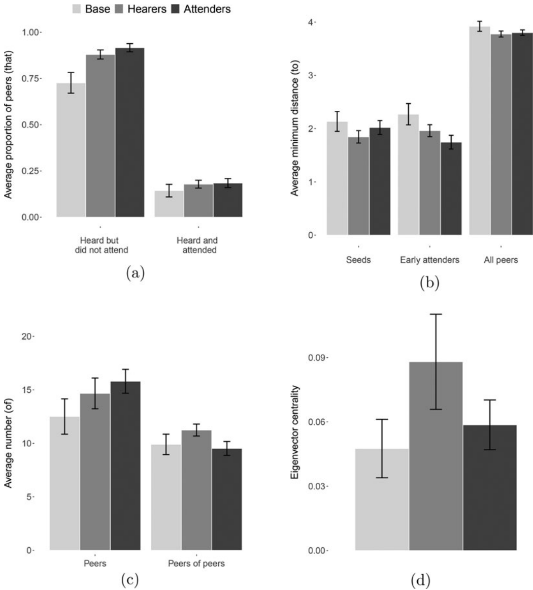
Fig. 2. Average and 95% confidence interval of various network measures grouped by hearing and attendance. Notes: Base are those who neither heard nor attended. Hearers are those who heard but did not attend. Attenders are those who both heard and attended the event. The same legend applies to all figures: (a) average proportion of peers that heard but did not attend and proportion of peers that heard and attended; (b) average distance to seeds, early attenders, and all peers; (c) average number of peers and peers of peers; and (d) eigenvector centrality.
