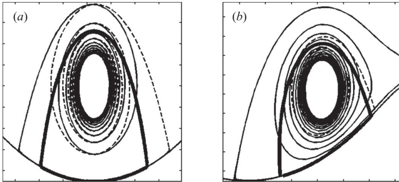
FIGURE 21. The stable (-----) and unstable (—) manifolds at (a) t/T = 1.0 and (b) t/T = 0.3 . Here, the separation bubble is shown as the thick solid line.
