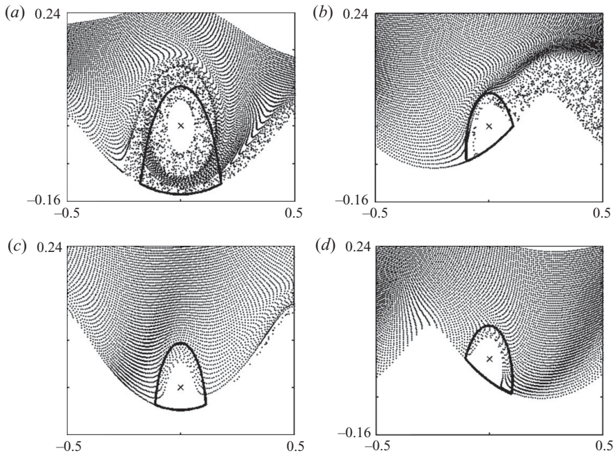
FIGURE 20. Instantaneous snapshots of particles' motion ( \bullet ) on a reference frame co-moving with the vortex ( \times ): (a) t/T = 0 or t/T = 1 ; (b)–(d) correspond to t/T = 0.4, 0.5 and 0.6 respectively. Note that the vacated zone in the vicinity of the vortex represents the vortex core (—, separation bubble).
