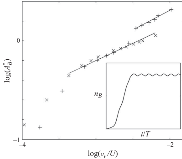
FIGURE 27. Power scaling law of the steady-state reactant front area: +, symmetrical channel; ×, skew-symmetrical channel. The inset shows typical temporal growth of the population of B particles inside the observation window.
