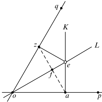
FIGURE 24. z = Rotate(p, o, q, a) . a is allowed to move along Line(o, p) , even through o .
