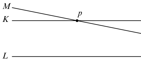
FIGURE 18. Playfair: M and L can’t fail to meet.
