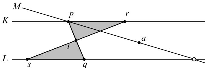
FIGURE 4. Strong Parallel Postulate: M and L must meet (somewhere) provided a is not on K and p is not on L and pt = qt and rt = st and r \neq p .
