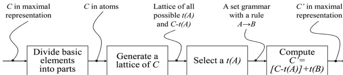
Fig. 1. Proposed method.
