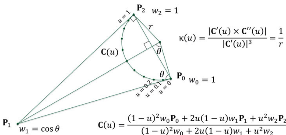
Fig. 3. Circular arc type basic element represented by a parametric curve C(u) with curvature \kappa(u) .
