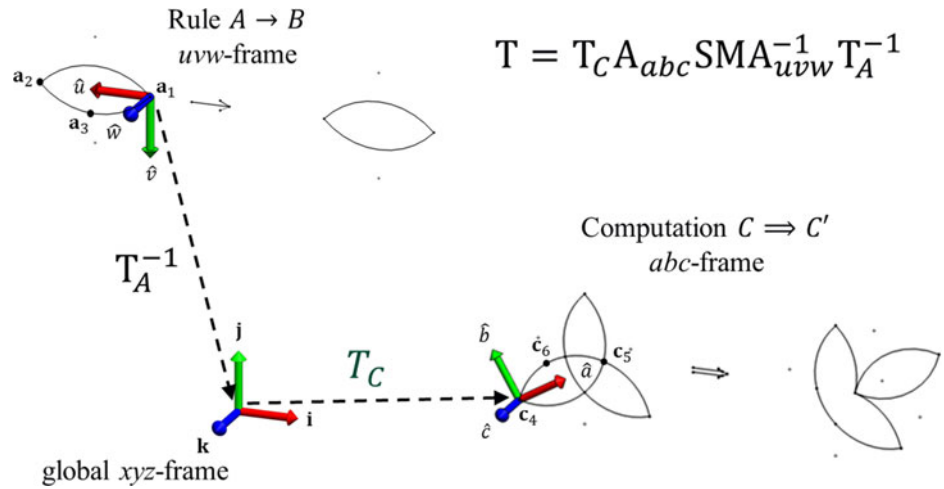
Fig. 4. A transformation t represented by a 4 \times 4 homogeneous matrix T .
