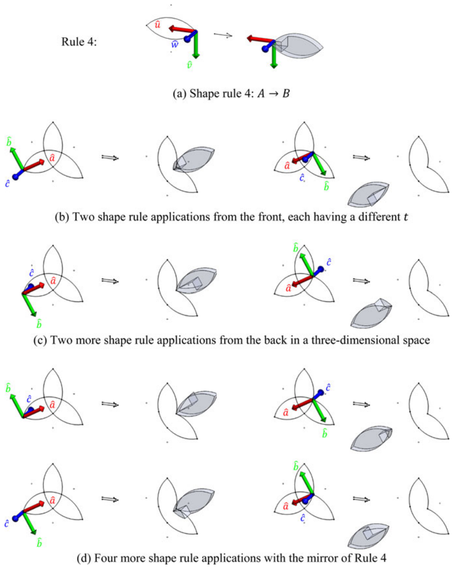
Fig. 14. Eight matching transformations t and eight corresponding resulting shapes t(B) for shape rule 4: A \rightarrow B .
