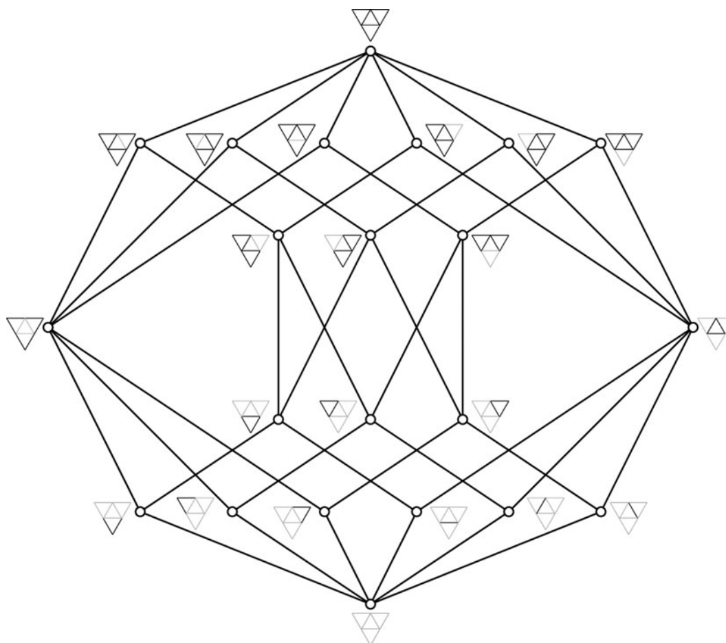
Fig. 8. Lattice of the initial shape C of the triangles grammar decomposed by Rule 1.
