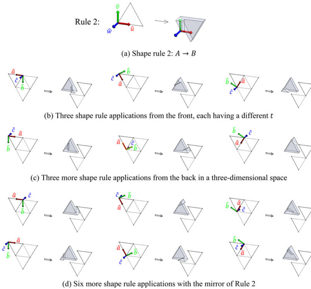
Fig. 13. Twelve matching transformations t and 12 corresponding resulting shapes t(B) for shape rule 2: A \rightarrow B .
