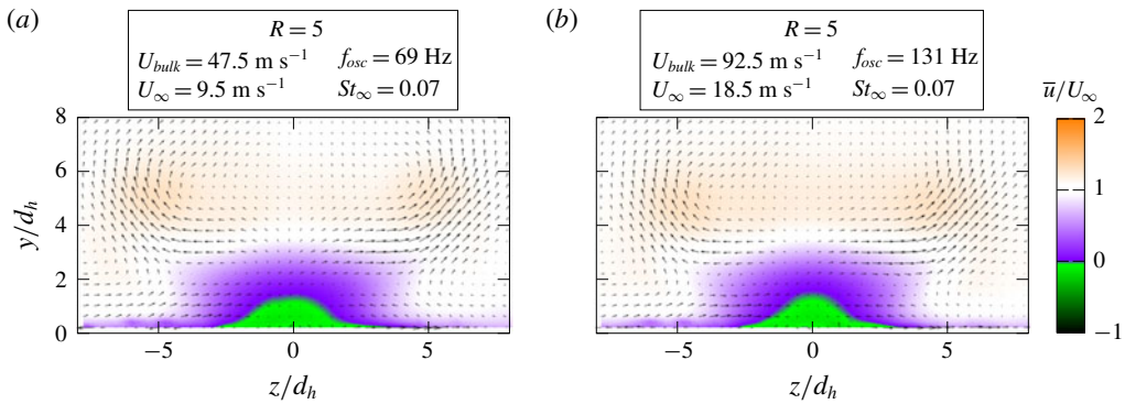
FIGURE 11. (Colour online) A cross-section through the time-averaged velocity field at x/d_h = 5.5 for two oscillation frequencies at the same velocity ratio.
