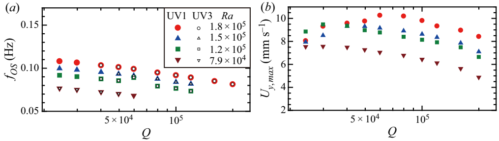
Figure 14. Variations of (a) the main frequency on the oscillatory convection, f_{OS} , obtained by UV1 and UV3, and (b) the maximum time-averaged velocity of the central convection rolls, U_{y,max} , in the five-roll state with respect to Q obtained at different Ra . In (a), the frequencies obtained by UV3 at most of the Q values agree with those by UV1 within the frequency resolution as overlaps of the solid and open symbols.
