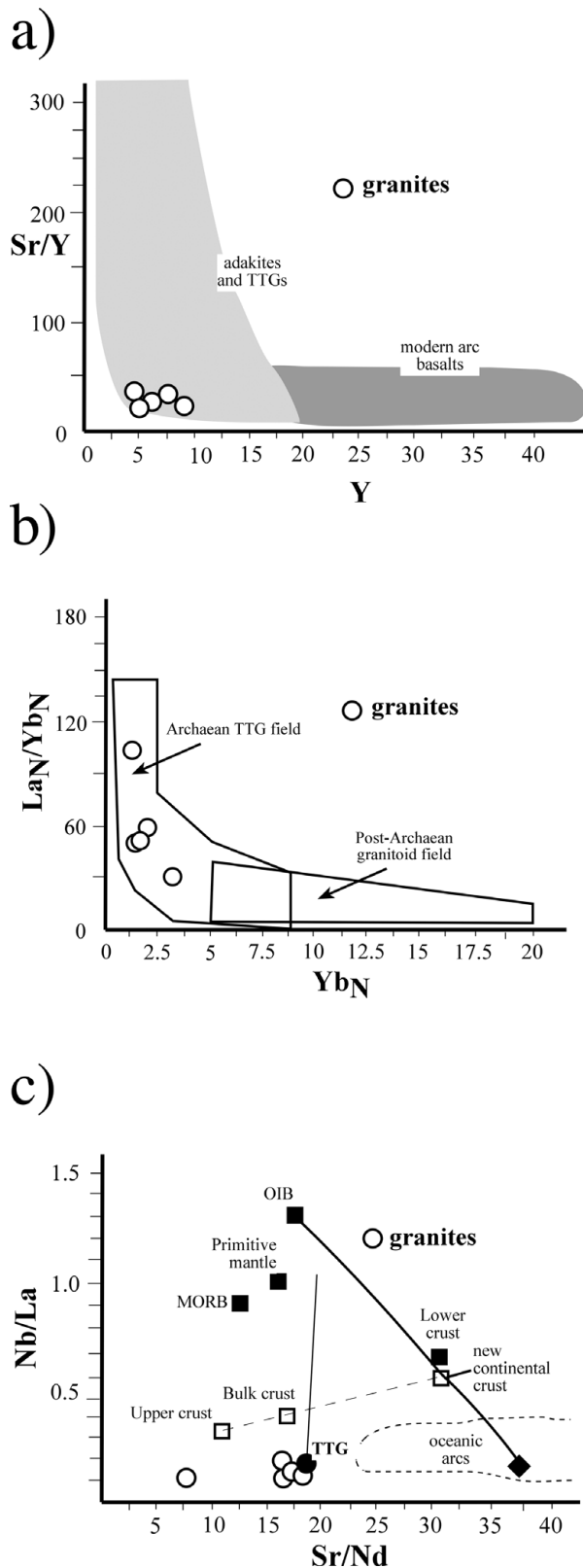
Figure 3. (a) Sr/Y versus Y diagram to decipher the type of granitic magma (Münker et al. 2004). (b) Plot of La/Yb versus Yb (normalized to chondrite, denoted by 'N') after Martin (1986). (c) Sr/Nd versus Nb/La ratios to characterize the magma composition. The samples plot very close to the typical TTG composition (Hawkesworth & Kemp, 2006).
