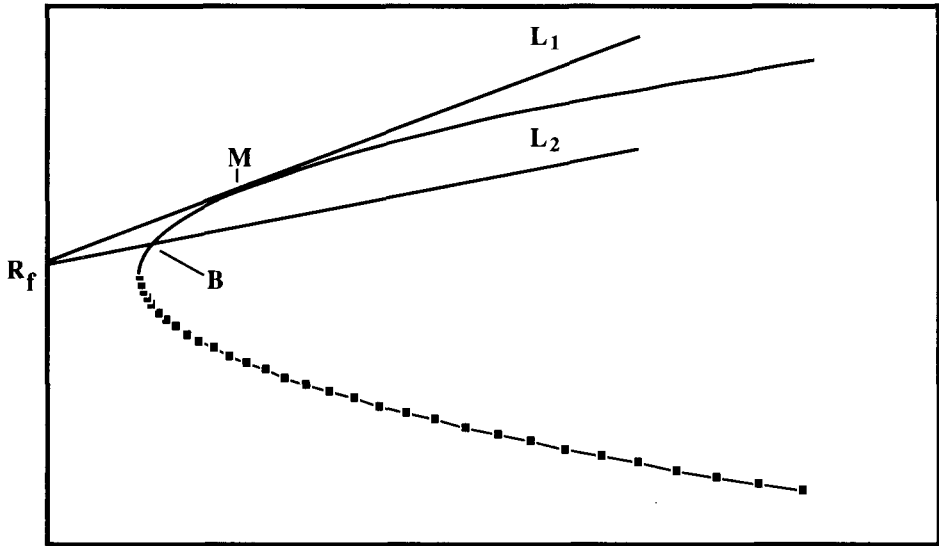
FIGURE 2. Two-fund separation.
