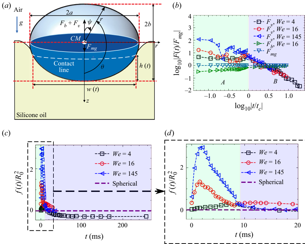
Figure 3. (a) Schematic representation depicting various geometrical scales and forces acting on the impacting droplet while it penetrates the silicone-oil pool; (b) log-log plot depicting the strength of various forces in comparison with weight of the droplet as a function of time normalized with respect to capillary time scale t_c = \sqrt{m/\sigma_{aw}} , where m is the mass of the droplet and \sigma_{aw} is the air–water surface tension with impact Weber number as a parameter; (c,d) f(t)/R_0^2 as a function of time in milliseconds. The function f(t) is a measure of a spherical drop shape.
