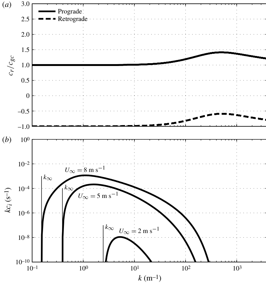
FIGURE 3. Three solutions of the dispersion relation (2.15) using the ‘double-exponential’ \mathcal{E}^* s in (4.8) and (4.9). The three solutions for c(k) = c_r(k) + ic_i(k) correspond to U_\infty = 2, 5 and 8 m s ^{-1} . (a) c_r(k) , normalized by c_{gc}(k) in (2.19); the three curves coincide to within the line width for both pro- and retrograde modes. (b) The growth rate kc_i . In this case, with U_s = c_{min}/2 , there is no rippling instability. The parameters in (4.1) are U_s = c_{min}/2 = 11.5 cm s ^{-1} , h_a = 1 m and h_w = 2/k_{min} = 0.54 cm.
