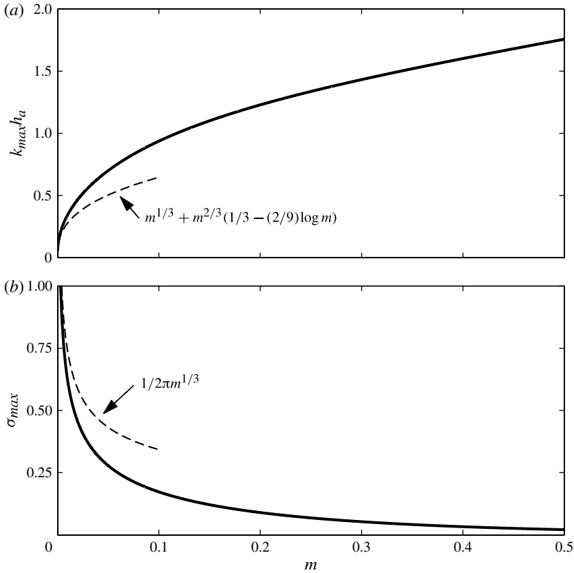
FIGURE 12. (a) The most unstable wavenumber as a function of m and (b) the maximum non-dimensional growth rate, \sigma_{max}(m) = \sigma(h_a k_{max}, m) . The dashed curves are the small- m approximations in (7.16) and (7.17).
