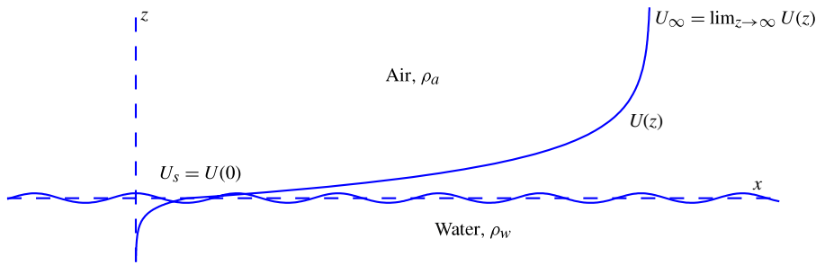
FIGURE 1. (Colour online) The coupled shear flow with the ‘double-exponential’ velocity profile in (4.1). Following Valenzuela (1976), the shear flow extends into the water with a shallow ‘wind-drift’ layer.
