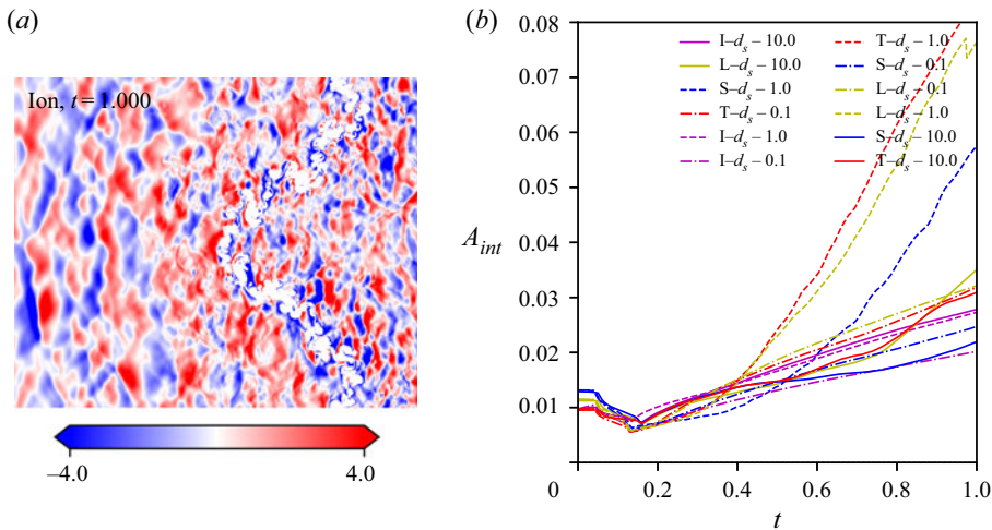
Figure 25. An example of the intense and alternating regions of Lorentz force causing the erratic interface statistics for a smoothly evolving interface area; (a) \lambda_D = 2 \times 10^{-2} He-3 SRMI x -Lorentz force at t = 1 with interface contour whited out and (b) interface area for all interface and skin depth scenarios.
