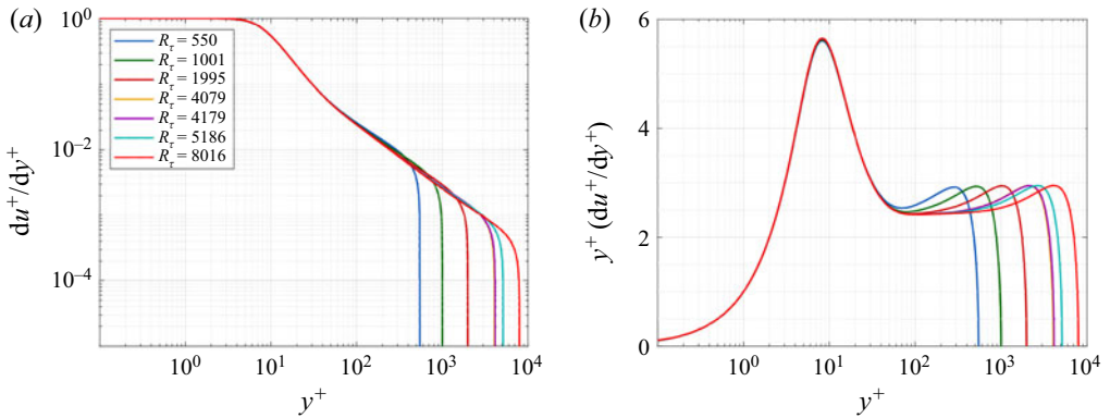
Figure 7. (a) Channel flow velocity gradient and (b) log indicator function at R_\tau values for channel flow DNS cases in table 3.
