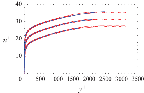
Figure 11. Optimal fit of the universal velocity profile (blue curves) to the data of Sillero et al. (2013) (open circles) for three choices of u_e/U . Curves and data are shifted vertically by 4 units for viewing. Upper curve u_e/U = 0.999 , R_\tau = 2471 , (k, a, m, b, n) = (0.4201, 25.1850, 1.1650, 0.1719, 2.2415) , u_{rms}^+ = 0.2074 ; middle curve u_e/U = 0.994 , R_\tau = 2088 , (k, a, m, b, n) = (0.4289, 25.9290, 1.1480, 0.1696, 2.2516) , u_{rms}^+ = 0.0314 ; lower curve u_e/U = 0.980 , R_\tau = 1834 , (k, a, m, b, n) = (0.4338, 25.8676, 1.1746, 0.1733, 2.3251) , u_{rms}^+ = 0.0805 .
