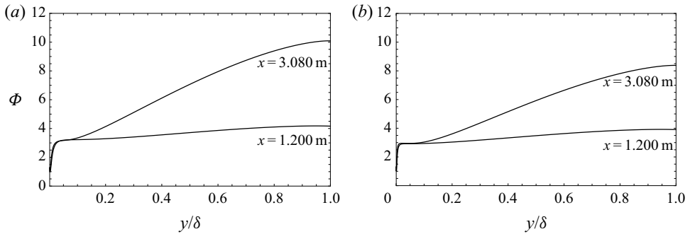
Figure 26. Boundary layer shape function from the universal profile at x = 1.2 and x = 3.08 m: (a) u_\infty = 10 \text{ m s}^{-1} and (b) u_\infty = 30 \text{ m s}^{-1} .
