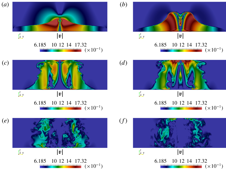
FIGURE 5. (Colour online) Time evolution of the velocity magnitude |\mathbf{v}| on the plane x_1 = 0 for the swirl case with Re = 50\,000 : t = 0.1 (a), 0.3 (b), 1.0 (c), 1.3 (d), 2.3 (e) and 3.0 (f).
