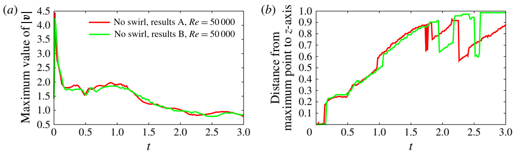
FIGURE 11. (Colour online) Graphs of (a) the maximum values of |\mathbf{v}| versus t and (b) the distance from the maximum point of |\mathbf{v}| to the z -axis versus t in the no-swirl case for Re = 50000 , where the red and green colours are employed for results A and results B, respectively.
