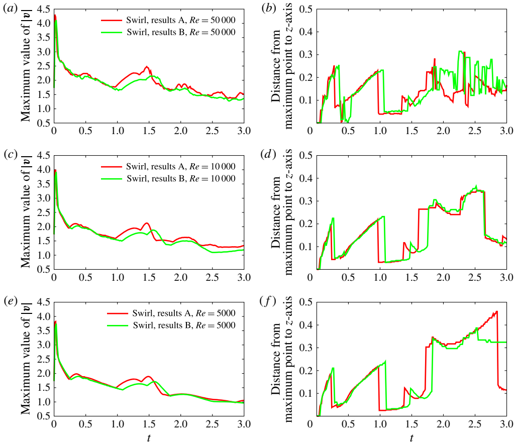
FIGURE 10. (Colour online) Graphs of (a,c,e) the maximum values of |\mathbf{v}| versus t and (b,d,f) the distance from the maximum point of |\mathbf{v}| to the z -axis versus t in the swirl case for Re = 50000 (a,b), 10000 (c,d) and 5000 (e,f), where the red and green colours are employed for results A and results B, respectively.
