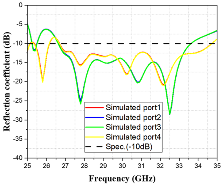
Figure 18. The reflection coefficient of the Butler matrix.
