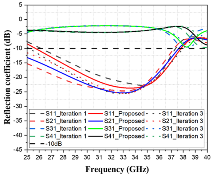
Figure 4. Simulated S-parameter of the hybrid coupler.
