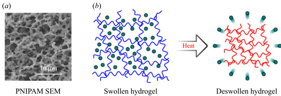
Figure 1. (a) A scanning electron microscope (SEM) image of the micro-structure of PNIPAM, reprinted from Ju et al. (2006) with permission from IOP Publishing. (b) Schematic of a thermo-responsive hydrogel's structure – as the gel is heated, it loses its affinity for the fluid in the pore space, hence it contracts and expels fluid.
