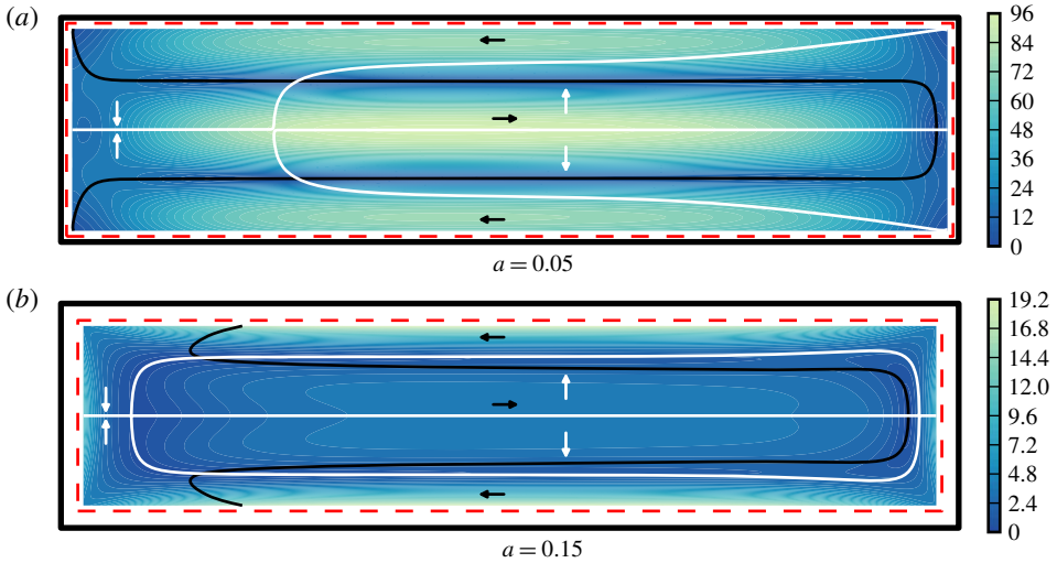
FIGURE 8. (Colour online) The force F'_p on neutrally buoyant particles at different locations in a curved duct with rectangular cross-section ( W/4 = H = 2 ) and bend radius R = 160 . The colour background shows the magnitude of F'_p . Black and white contours are the zero level set curves of the horizontal and vertical components, respectively, whereas the arrows indicate the sign of each component in the area bounded by the respective contour. The left wall is on the inside of the bend. The dashed red line shows where the centre of the particle lies when its surface touches the wall.
