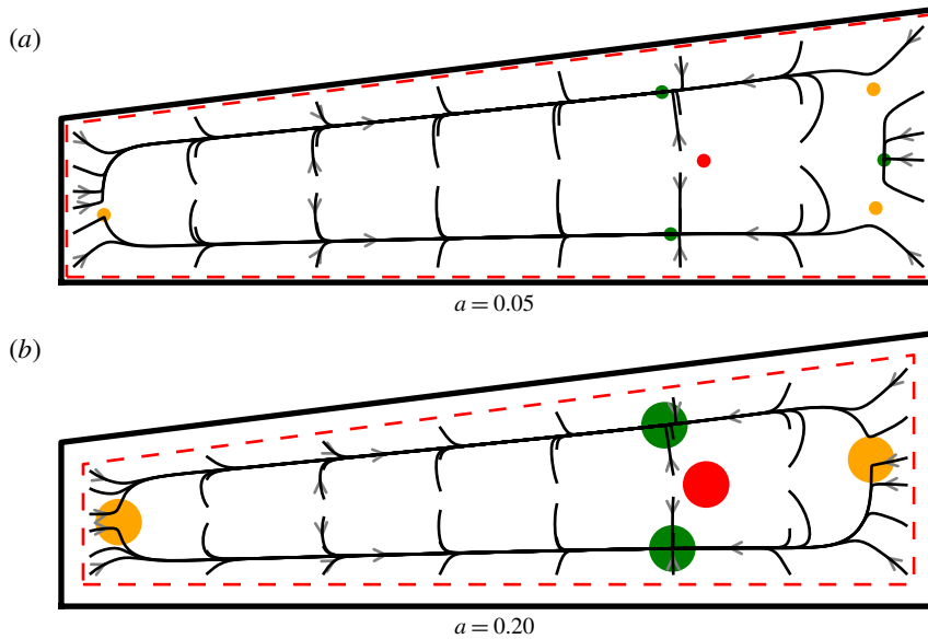
FIGURE 21. (Colour online) Approximate trajectories of neutrally buoyant particles in a straight duct with trapezoidal cross-section ( W = 8 , H_{left} = 3/2 and H_{right} = 5/2 ). Trajectories from several starting positions are superimposed. Green, orange and red markers show the location of stable, (unstable) saddle and unstable equilibria, respectively (with marker size indicative of particle size). The dashed red line shows where the centre of the particle lies when its surface touches the wall.
