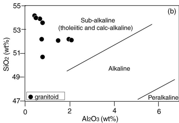
Figure 9. (a) Ti (a.p.f.u.) against Na+Ca (a.p.f.u.) diagram (Leterrier et al. 1982). (b) Sub-alkaline characteristic of the granitoids on the SiO_2 (wt%)– Al_2O_3 (wt%) diagram. The positions of boundaries between sub-alkaline, alkaline and peralkaline magma types are from Le Bas (1962).
