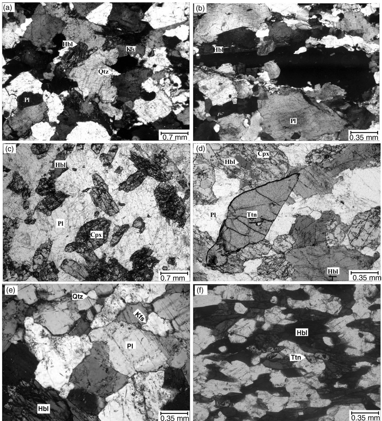
Figure 4. (a) Hornblende and plagioclase with granular texture in the granodiorite. Plagioclase shows compositional zoning. Crossed nicols, field of view 4.8 mm. (b) Subsolidus actinolite around magmatic hornblende in the granodiorite. Plain polarized light, field of view 2.4 mm. (c) Clinopyroxene, amphibole and plagioclase in the quartz diorite. Subsolidus amphibole is seen parallel to the cleavage system of clinopyroxene. Plain polarized light, field of view 2.4 mm. (d) Magmatic titanite in the diorite. Amphibole as patches within clinopyroxene and as products of deuteritic alteration. Plain polarized light, field of view 2.4 mm. (e) The migmatitic leucosome with granular texture. Interstitial quartz and K-feldspar are anhedral. Plain polarized light, field of view 2.4 mm. (f) Hornblende and plagioclase with foliated texture in the mesosome. Plain polarized light, field of view 2.4 mm.
