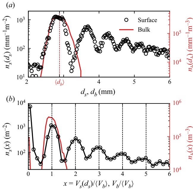
Figure 18. Distributions, for clean water, of bubbles at the surface ( n_s (left-hand axis, black symbols) and in the bulk n_b (right-hand axis, red) for a low flow rate q_v = 25 \text{ cm}^3 \text{ min}^{-1} . (a) Size distributions n_s(d_s) and n_b(d_b) . The vertical dotted line indicates the bulk bubble mean size \langle d_b \rangle . (b) Volume distributions n_s(V_s(d_s)/\langle V_b \rangle) and n_b(V_b/\langle V_b \rangle) , where volumes are normalized by the bulk bubble volume \langle V_b \rangle = \pi \langle d_b^3 \rangle / 6 . Vertical dotted lines are located at integer values of \langle V_b \rangle and highlight corresponding peaks in the distribution n_s(V_s/\langle V_b \rangle) .
