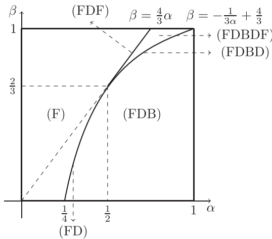
Figure 1. Classification of equation (1.9).
