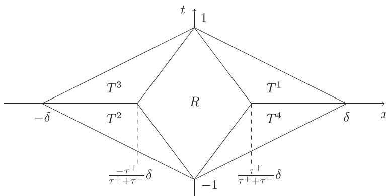
Figure 4. Five disjoint domains T^1, T^2, T^3, T^4, R \subset D in lemma 7.1.
