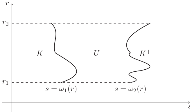
Figure 3. The right wall K^+ and left wall K^- .
