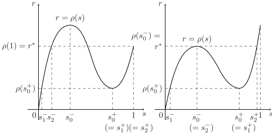
Figure 2. Two possible graphs of r = \rho(s) ( 0 \leq s \leq 1 ).
