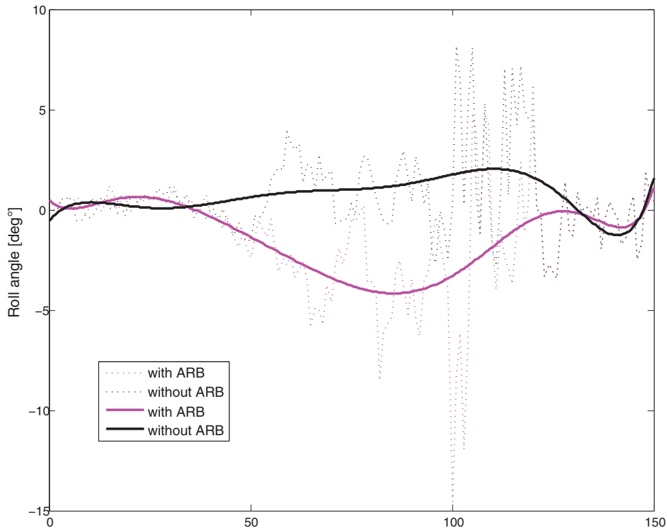
Fig. 21. Roll angle at 8 m/s as a function of time.
