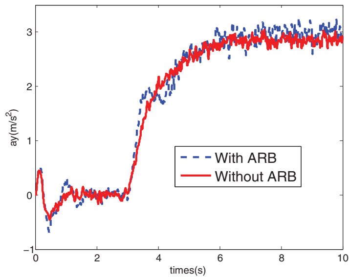
Fig. 14. Lateral acceleration with respect to time.
