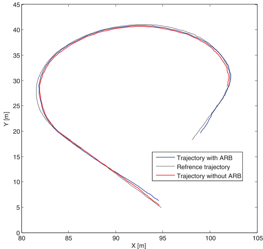
Fig. 18. Trajectory at 5 m/s.
