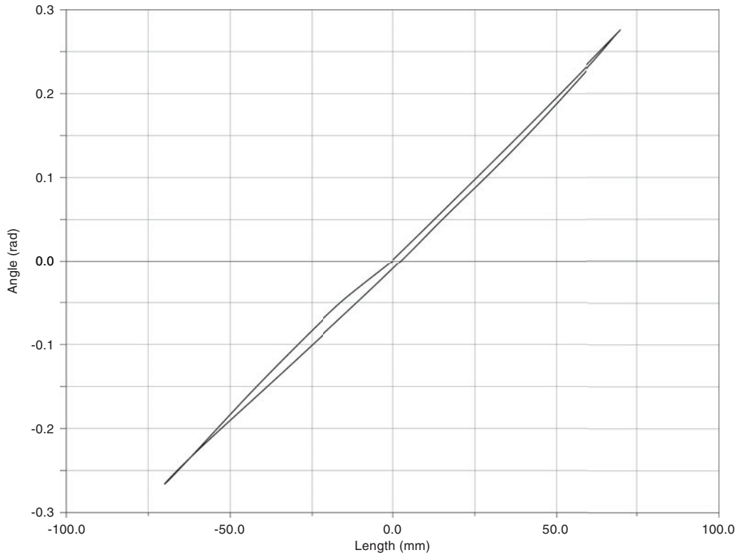
Fig. 4. Mechanical characteristics of the first kinematic configurations: horizontal actuator on the left. Relationship between roll angle and linear actuator displacement.
