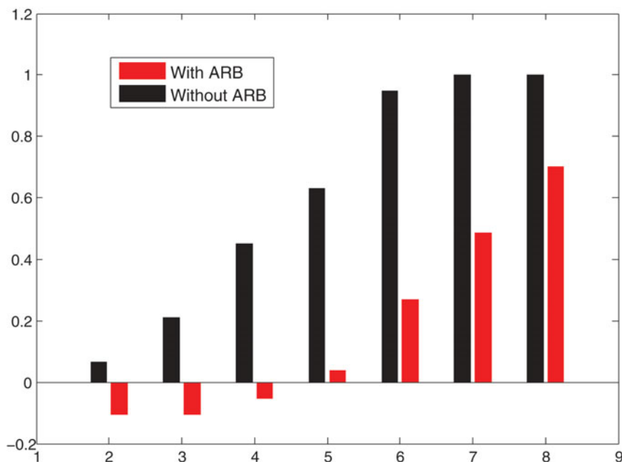
Fig. 17. Normalized lateral load transfer as a function of robot speed.
