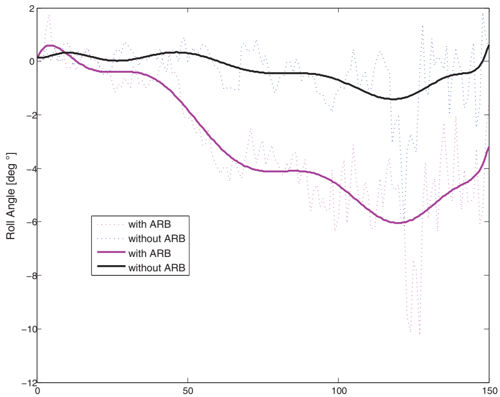
Fig. 20. Roll angle at 5 m/s as a function of time.
