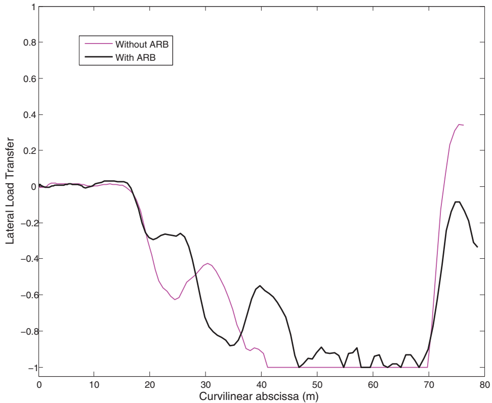
Fig. 23. Normalized lateral load transfer LLT at 8 m/s.
