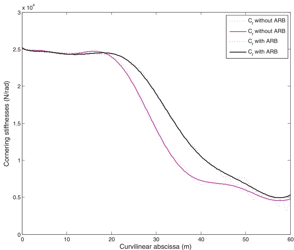
Fig. 26. Cornering stiffness at the rear of the robot at 5 m/s.
