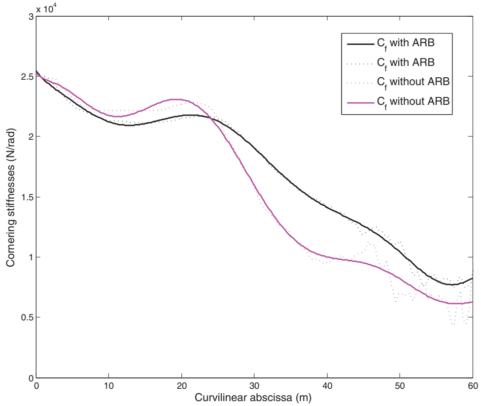
Fig. 27. Cornering stiffness at the front of the robot at 5 m/s.
