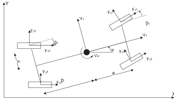
Fig. 8. A four-wheeled vehicle with front steering.
