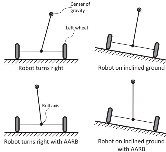
Fig. 1. Alternative kinematic configuration for the active anti-roll mechanism.
