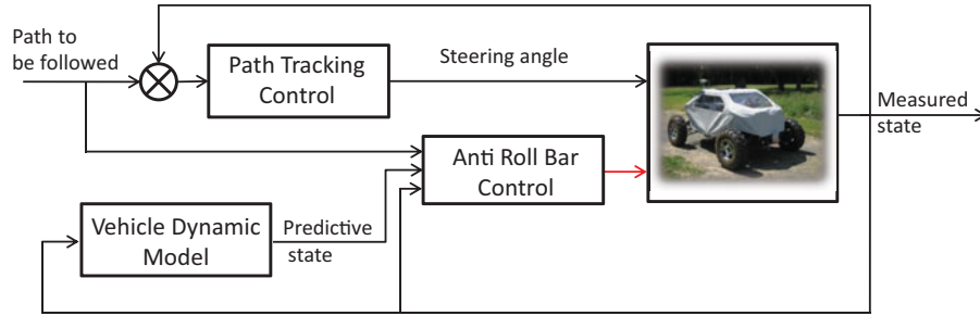
Fig. 10. Block diagram for the proposed model predictive controller.
