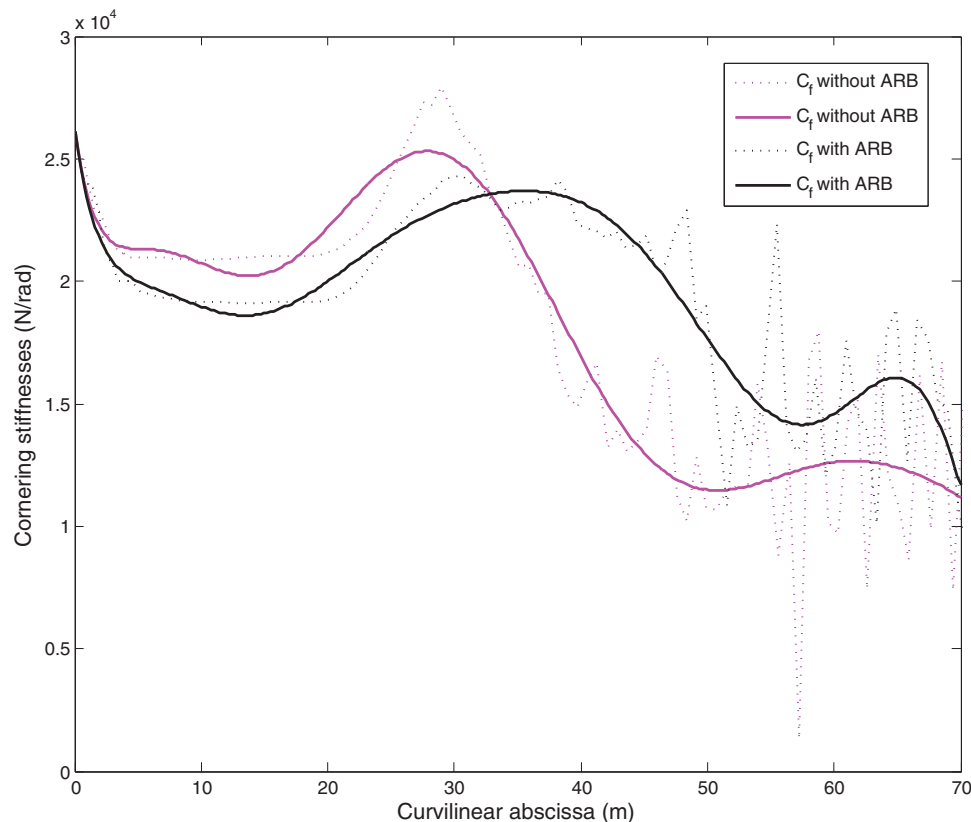
Fig. 29. Cornering stiffness at the front of the robot at 8 m/s.
