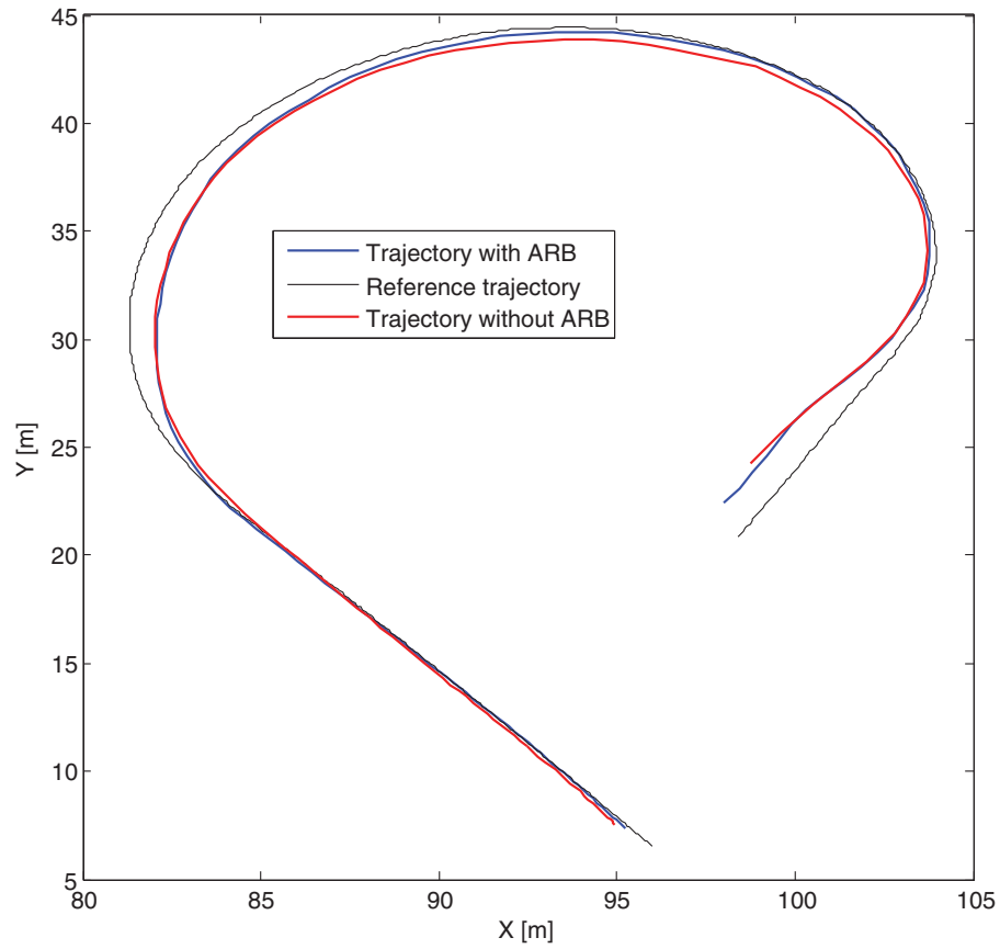
Fig. 19. Trajectory at 8 m/s.
