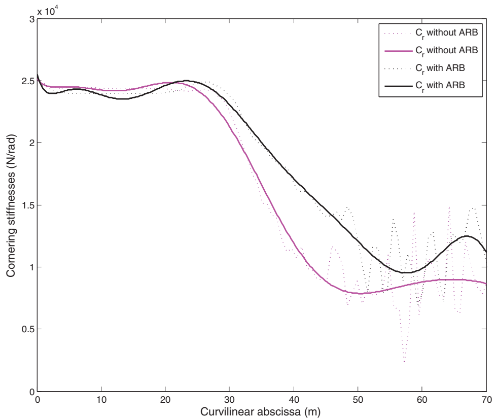
Fig. 28. Cornering stiffness at the rear of the robot at 8 m/s.
