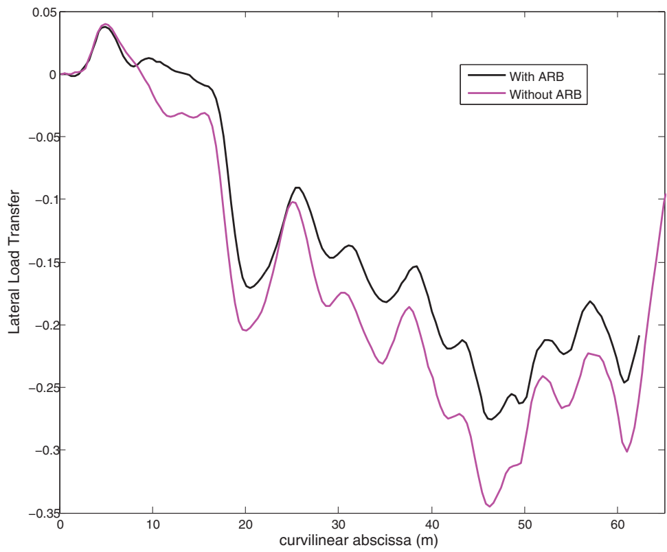
Fig. 22. Normalized lateral load transfer LLT at 5 m/s.
