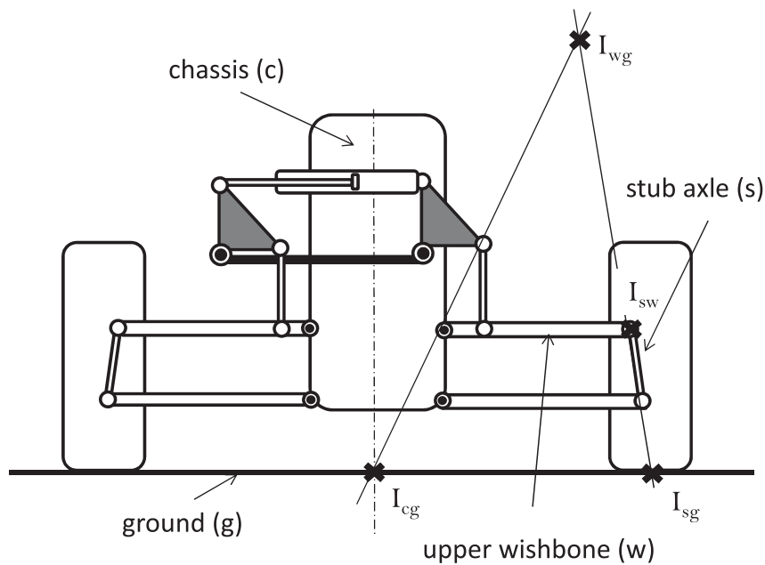
Fig. 5. Location of the instantaneous centers of rotation.
