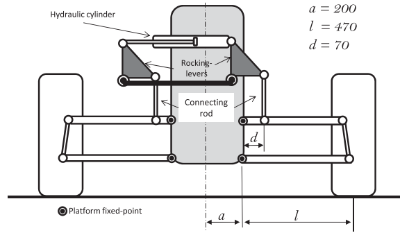
Fig. 2. Kinematics of the active anti-roll mechanism.
