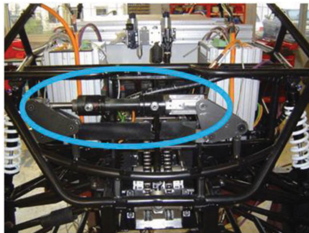
Fig. 7. Anti-roll device mounted on the rover.
