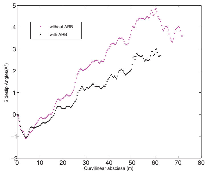
Fig. 24. Slip angle at 5 m/s.
