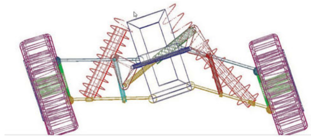
Fig. 3. Alternative kinematic configuration for the active anti-roll mechanism.
