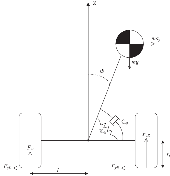
Fig. 9. Vehicle model in the roll direction.
