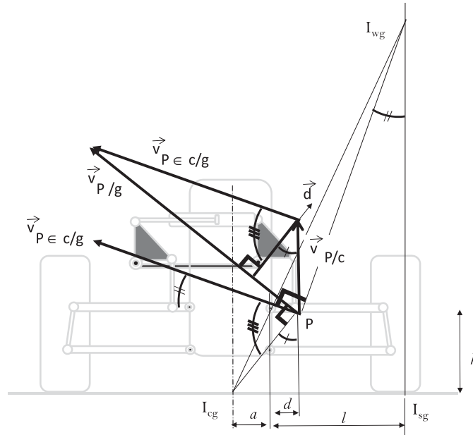
Fig. 6. Composition of the linear velocity of point P , using the relative velocity formula.
