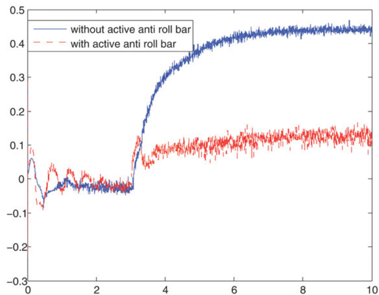
Fig. 15. LLT with respect to time.
