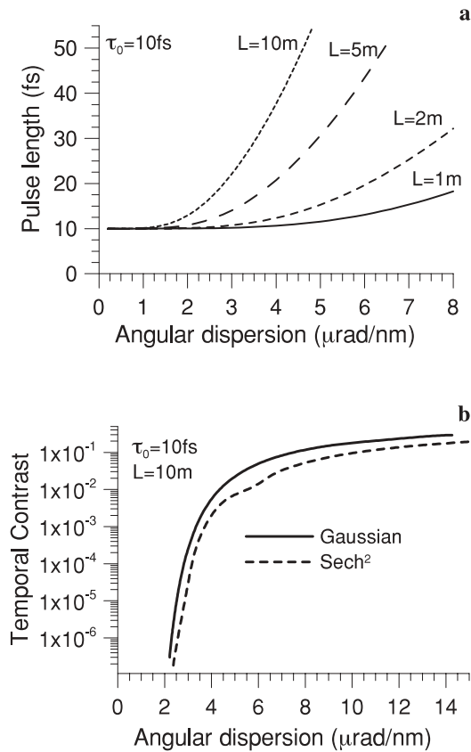
Fig. 4. Temporal broadening (a) and contrast degradation (b) of a transform limited 10 fs pulse in the function of angular dispersion after propagating L distance from the angular disperser.
