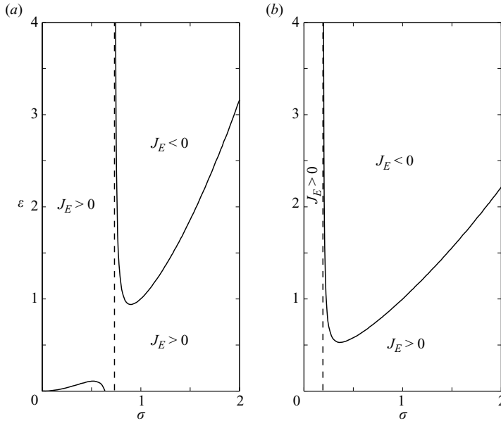
FIGURE 2. Long-wave analysis. The curve J_E = 0 is represented in the (\epsilon, \sigma) -plane for two cases where \mu > n^2 : (a) \mu = 2, n = 0.8 ; (b) \mu = 0.25, n = 0.2 .
