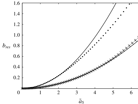
FIGURE 14. The value of b_{res} for j = \{4, 5\} (crosses) and for j = \{4, 5, 2\} (dots) for increasing \tilde{a}_5 . The solid lines are proportional to \tilde{a}_5^2 . Parameter values as in Ding & Umbanhowar (2006) but with \tilde{\nu} = 0.21 \text{ cm}^2 \text{ s}^{-1} .
