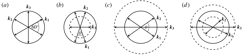
FIGURE 4. Possible spatial three-wave resonant interactions defined such that \mathbf{k}_1 + \mathbf{k}_2 = \mathbf{k}_3 . (a) |\mathbf{k}_1| = |\mathbf{k}_2| = |\mathbf{k}_3| ; (b) |\mathbf{k}_1| = |\mathbf{k}_2| > |\mathbf{k}_3| ; (c) |\mathbf{k}_1| = |\mathbf{k}_2| < |\mathbf{k}_3| ; (d) |\mathbf{k}_1| \neq |\mathbf{k}_2| \neq |\mathbf{k}_3| .
