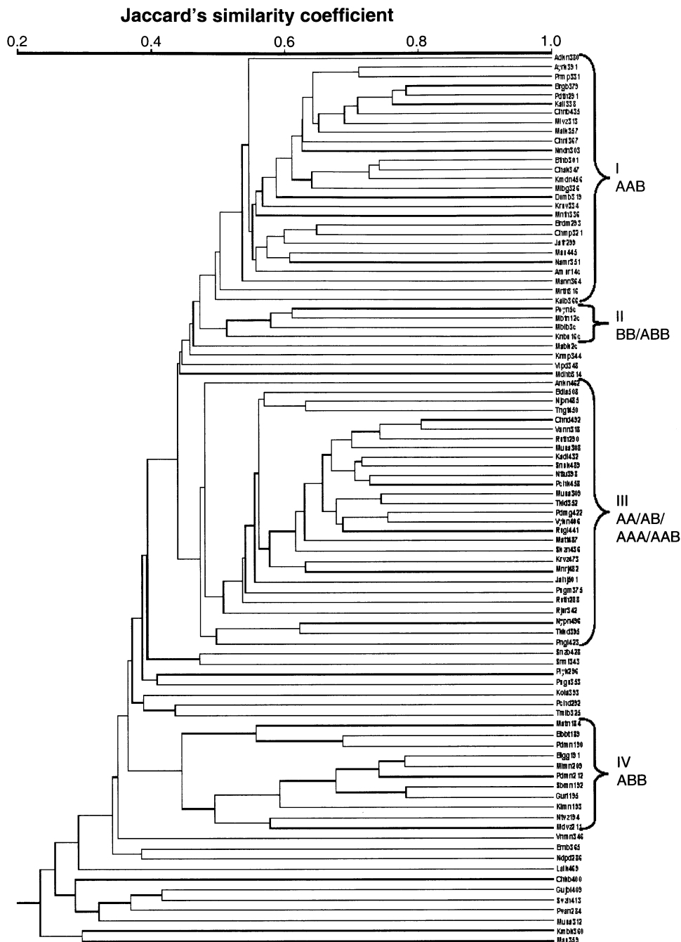
Fig. 2. UPGMA dendrogram depicting the diversity and relationships among Indian banana and plantain cultivars.
