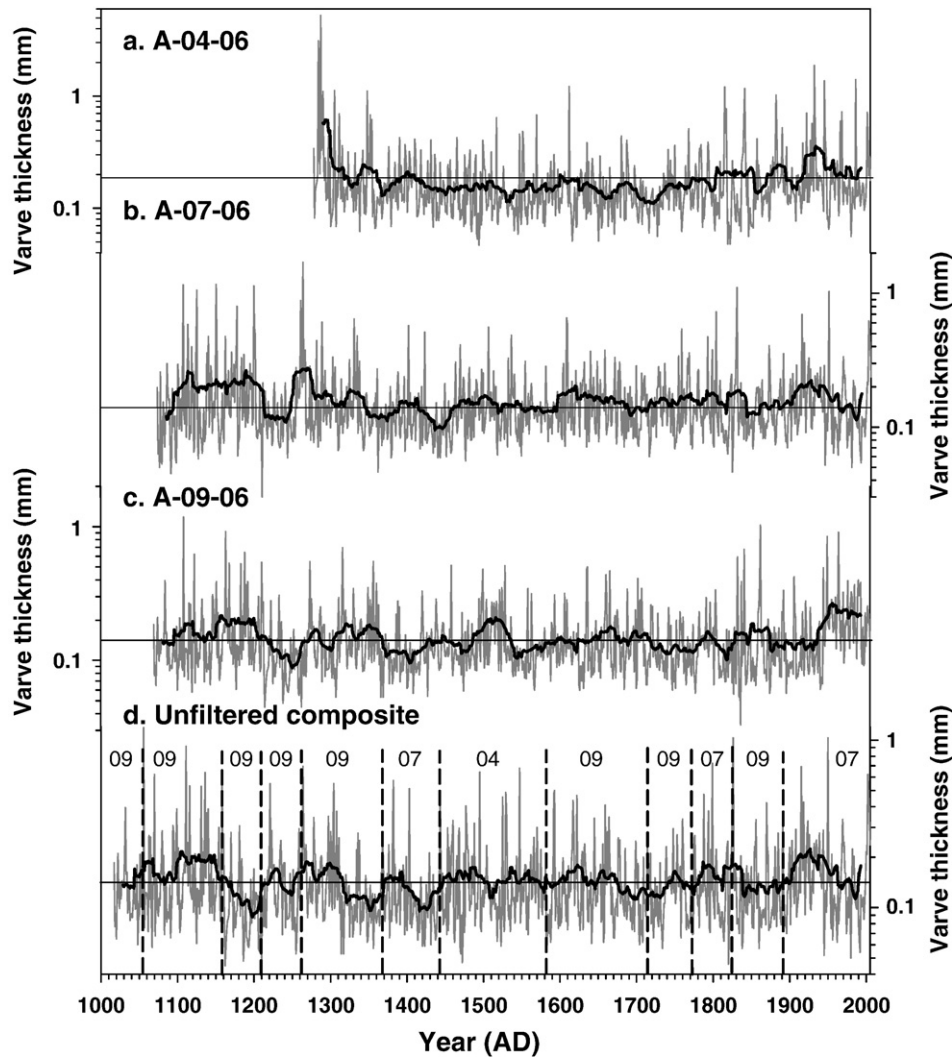
Figure 4. Unfiltered varve-thickness records from cores (a) A-04-06, (b) A-07-06, and (c) A-09-06 and (d) the unfiltered composite varve-thickness record that incorporates varve-thickness values from all three cores (indicated by 04, 07, and 09), plotted on a base-10 logarithmic scale. Dashed lines indicate marker beds, thin black lines indicate mean varve-thickness for each core and thick black lines indicate 25-yr unweighted moving means.
