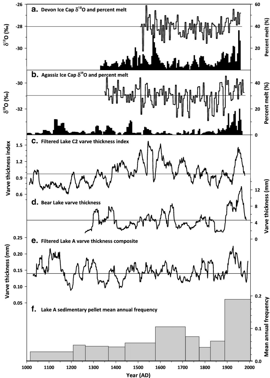
Figure 7. Comparison of regional paleoclimate records including (a) Devon Island Ice Cap \delta^{18}\text{O} (annual and 25-yr unweighted moving mean) and percent melt records (5-yr means; core A77, Fisher and Koerner, 1994; Fisher et al., 1995), (b) Agassiz Ice Cap \delta^{18}\text{O} (annual and 25-year unweighted moving average) and percent melt records (5-yr means; 1973 core, Fisher et al., 1983), (c) Lake C2 filtered varve thickness index (25-yr unweighted moving mean, Lamoureux and Bradley, 1996), (d) Bear Lake varve thickness (25-yr unweighted moving mean, Lamoureux and Gilbert, 2004), (e) Lake A filtered varve thickness composite (25-yr unweighted moving mean), and (f) Lake A mean annual ice-rafted pellet frequency (Tomkins et al., 2009b). Data for (a) and (b) was obtained from the IGBP PAGES/World Data Center for Paleoclimatology, NOAA/NGDC Paleoclimatology Program ( http://www.ncdc.noaa.gov/paleo/data.html ).
