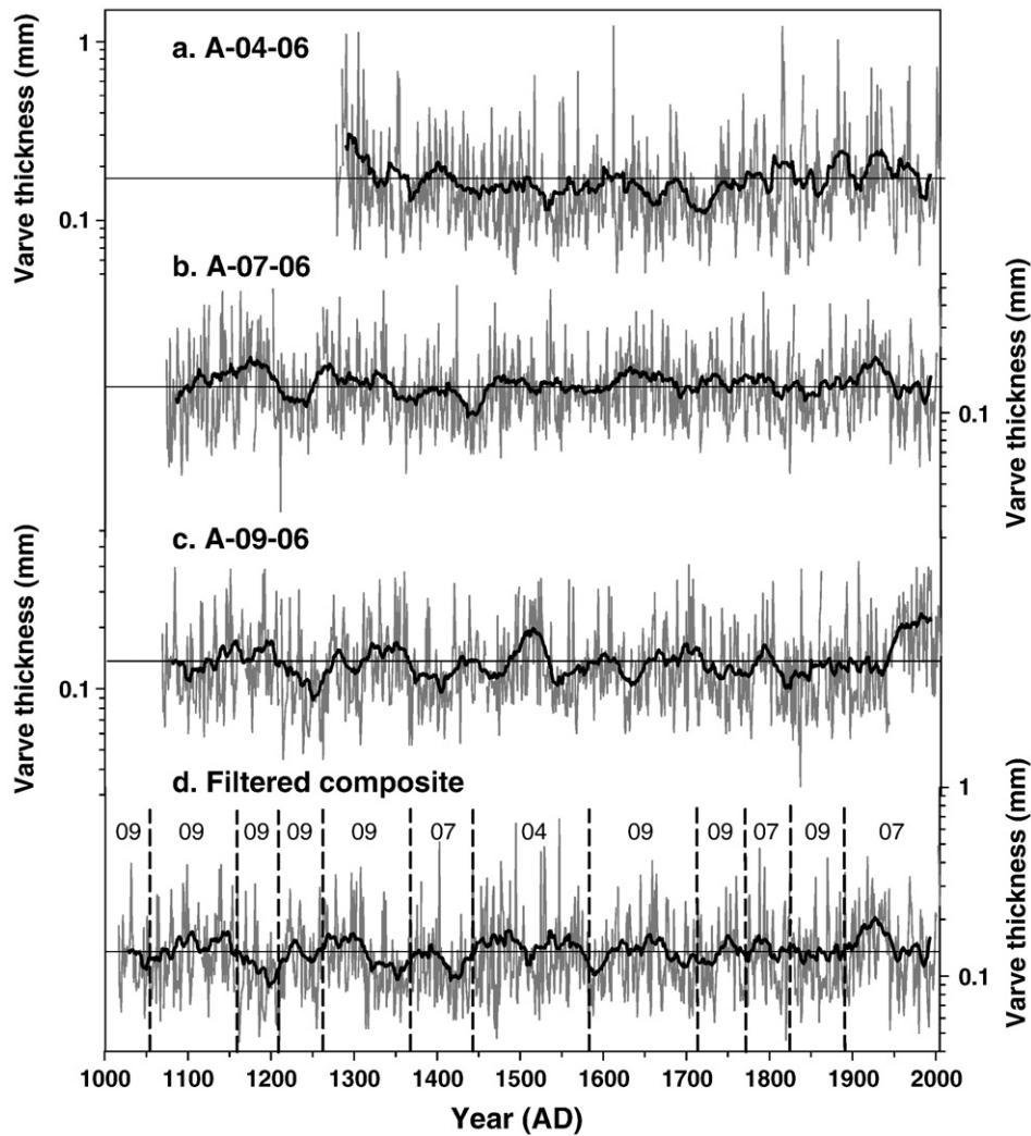
Figure 5. Filtered varve thickness records from cores (a) A-04-06, (b) A-07-06, and (c) A-09-06 and (d) the filtered composite varve thickness record that incorporates varve thickness values from all three records (indicated by 04, 07, and 09), plotted on a base-10 logarithmic scale. Dashed lines indicate marker beds, thin black lines indicate mean varve thickness for each core, and black lines indicate 25-yr unweighted moving means.
