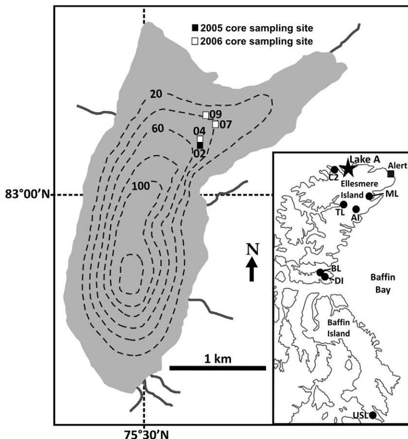
Figure 1. Lake A bathymetry (in metres) and location relative to meteorological records at Alert and other paleoclimate records discussed in the text (inset map; AI = Agassiz Ice Cap, BL = Bear Lake, C2 = Lake C2, DI = Devon Island Ice Cap, ML = Murray Lake, TL = Tuborg Lake and USL = Upper Soper Lake). Sampling locations of cores discussed in text are also shown.
