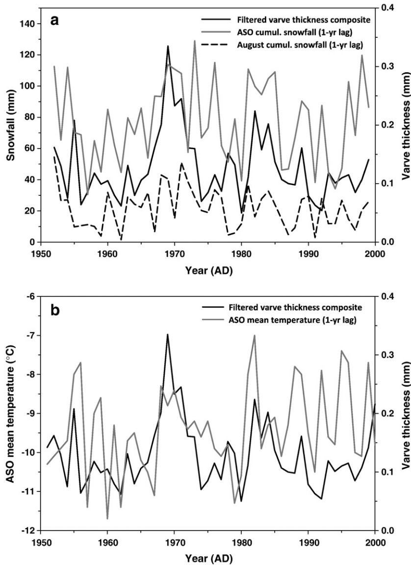
Figure 6. Comparison of the Lake A filtered varve thickness composite record with (a) August and combined August, September, and October (ASO) cumulative daily snowfall records (lagged 1 yr) and (b) the ASO mean daily temperature record (lagged 1 yr) from Alert, Nunavut.
