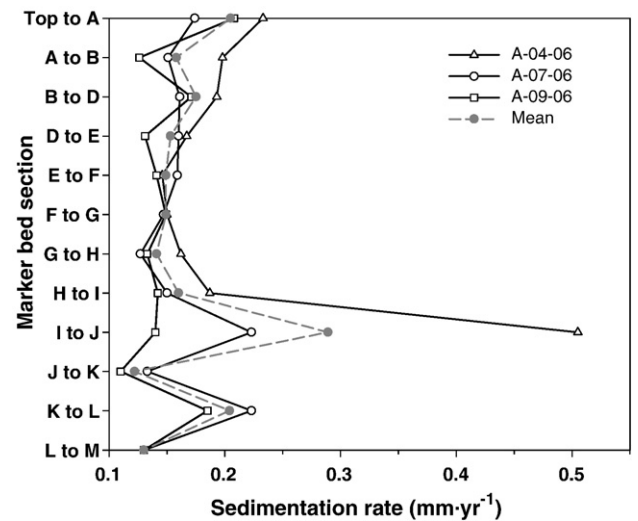
Figure 3. Sedimentation rates between marker beds in cores A-04-06, A-07-06, and A-09-06 and mean sedimentation rates for all three cores. Marker bed C was not included due to its close proximity to marker bed B and marker beds K and L in core A-04-06 were not clearly discernable.
