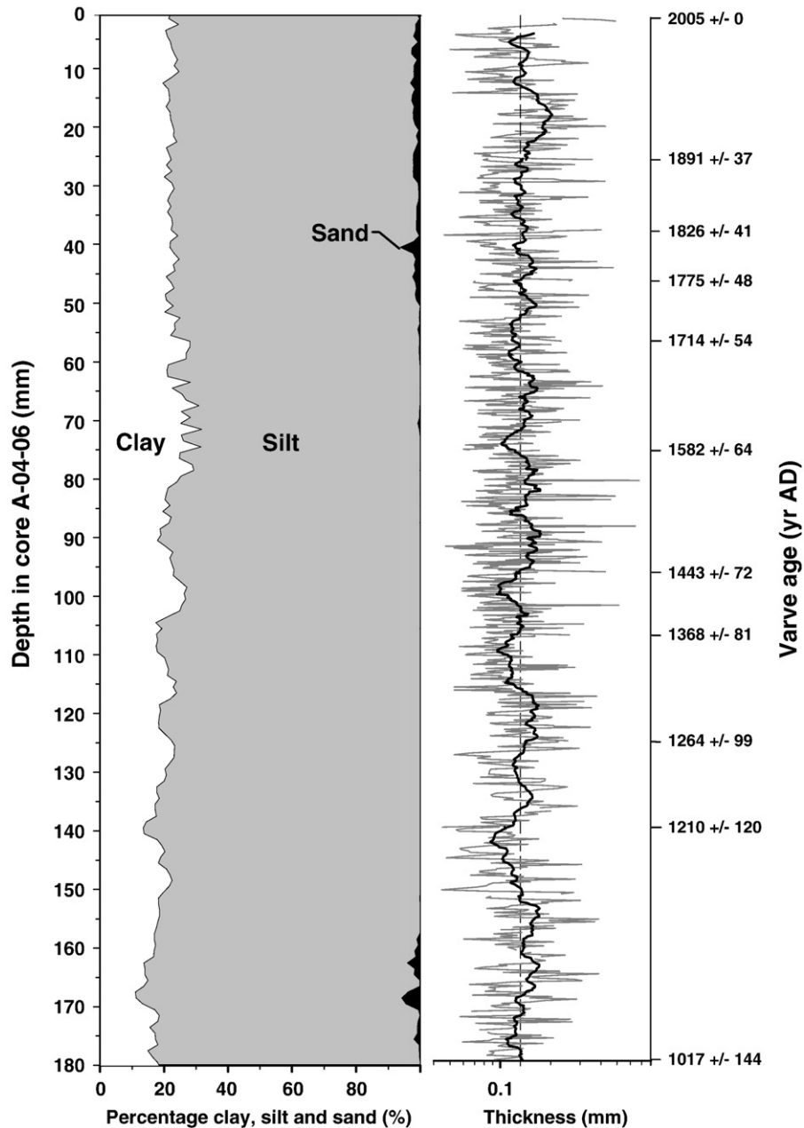
Figure 2. Grain size data from the varved section of core A-04-06. Dates are given for core A-04-06 by fitting the filtered composite varve thickness record to marker beds and date error estimates were derived from an age–depth model (Tomkins et al., 2009a). Mean varve thickness is denoted by the grey dashed line and varve thickness is plotted on a base-10 logarithmic scale.
