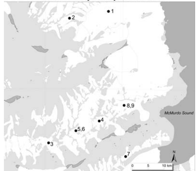
Fig. 1. Overview map of the study area. 1 = Victoria Lower Glacier, 2 = Baldwin Valley Glacier, 3 = Rhone Glacier, 4 = Canada Glacier, 5 = Newall Glacier (1), 6 = Newall Glacier (2), 7 = Howard Glacier, 8 = Commonwealth Glacier (1), 9 = Commonwealth Glacier (2).
