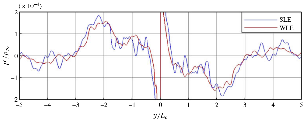
FIGURE 5. (Colour online) The profiles of perturbed pressure taken from figure 4 along a vertical line at (x, z) = (-0.5L_c, 0) showing the reduced small-scale fluctuations in the WLE case.
