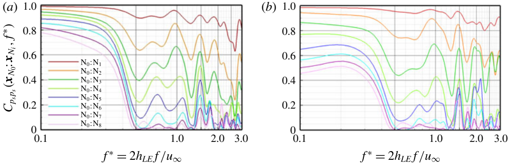
FIGURE 21. (Colour online) Two-point coherence spectra (magnitude squared) of surface pressure fluctuations along the LE; C_{p_s p_s}(\mathbf{x}_{N_0} : \mathbf{x}_{N_i}, f) for i = 1, \dots, 8 ; between the peak ( N_0 ) and the remaining probe points ( N_1, \dots, N_8 ) denoted in figure 15, for the (a) SLE and (b) WLE cases. The WLE case is for h_{LE}/L_c = 1/15 and \lambda_{LE}/L_c = 2/15 .
