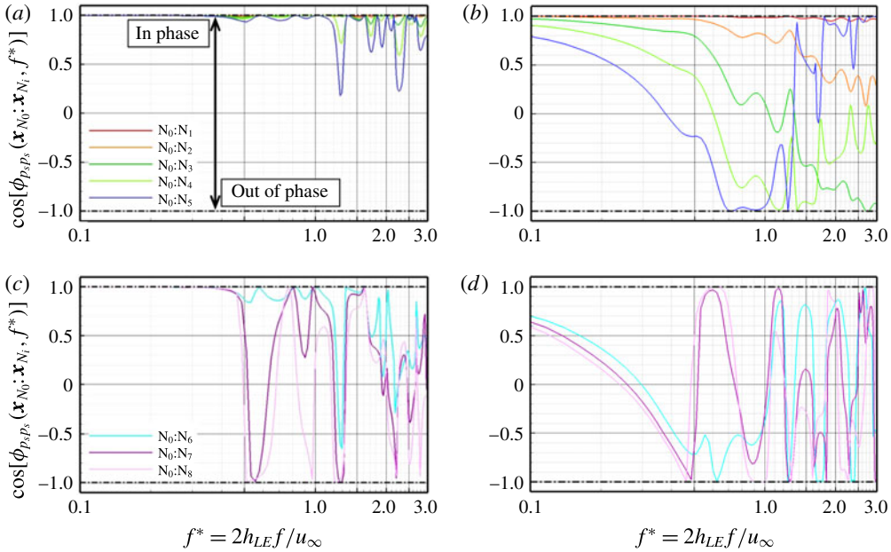
FIGURE 22. (Colour online) The profiles of \cos[\phi_{p_s p_s}(\mathbf{x}_{N_0} : \mathbf{x}_{N_i}, f^*)] where \phi_{p_s p_s}(\mathbf{x}_{N_0} : \mathbf{x}_{N_i}, f) is the two-point phase spectrum of surface pressure fluctuations between the peak ( N_0 ) and one of the remaining probe points ( N_1, \dots, N_8 ) denoted in figure 15, for the (a,c) SLE and (b,d) WLE cases. The WLE case is for h_{LE}/L_c = 1/15 and \lambda_{LE}/L_c = 2/15 .
