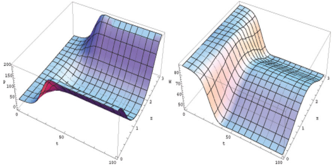
Figure 1. Pattern formation in plant biomass and groundwater
